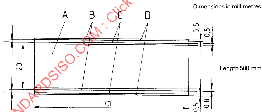
Figure 1 — Dimensions and design of the test assembly
