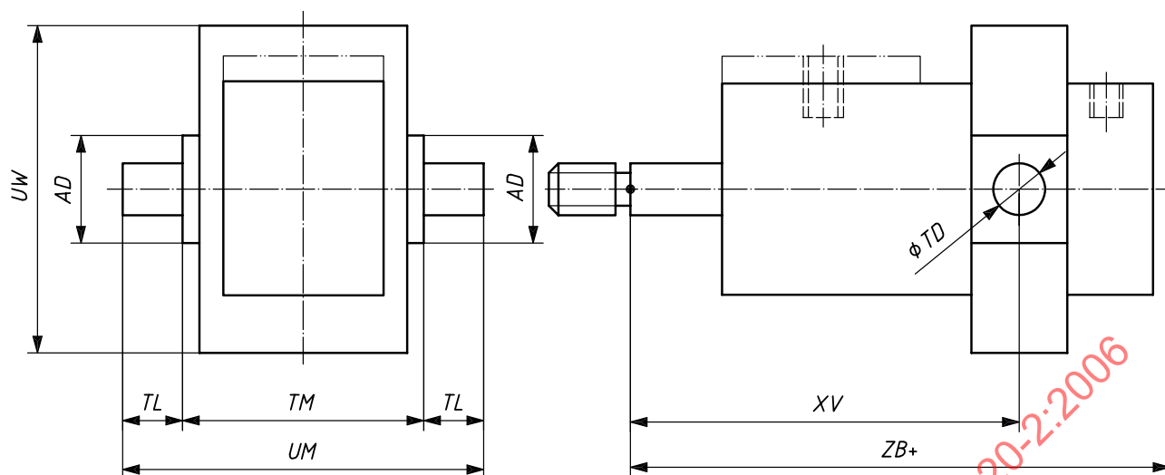
Figure 10 — MT 4 — Intermediate fixed or movable trunnion (male)
