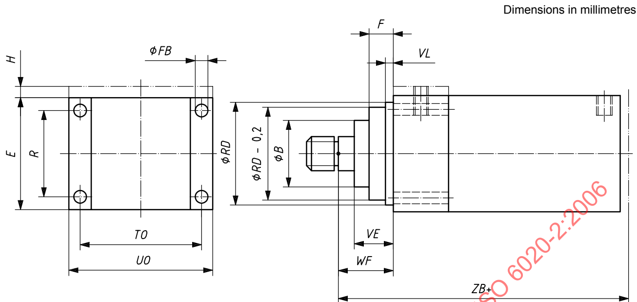
Figure 2 — ME 5 — Head, rectangular
