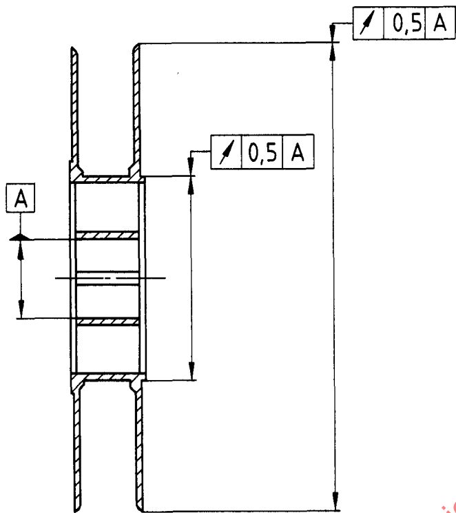
Figure 2 — Maximum radial runout
