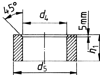
Figure 8 — Shape of bearing eye, form D
