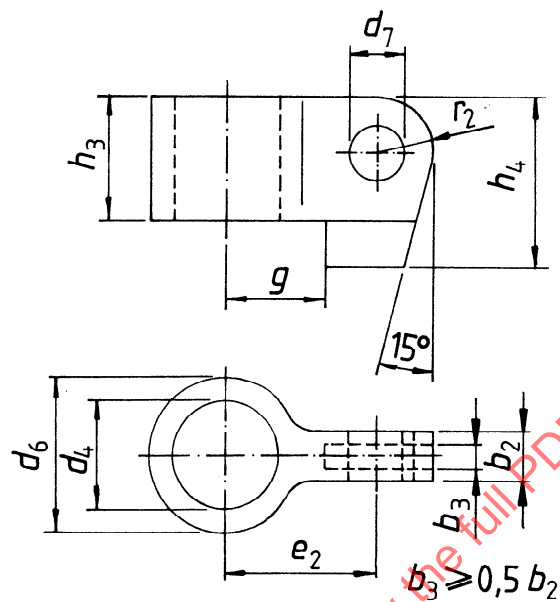
Figure 10 — Shape of lead block holder, form F
