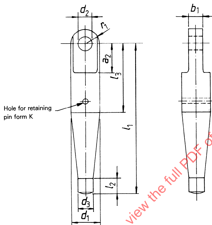
Figure 7 — Shape of gooseneck pin, form GC
