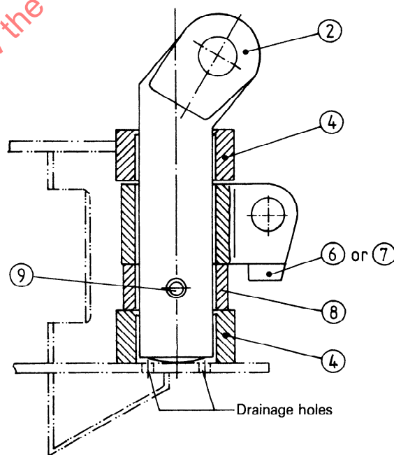
Figure 2 — Illustration of type B assembly
