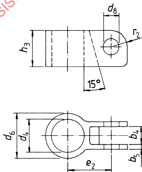
Figure 11 — Shape of lead block holder, form H
