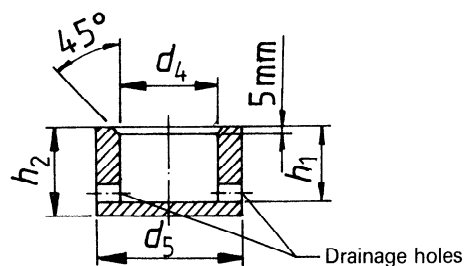
Figure 9 — Shape of bearing eye, form E
