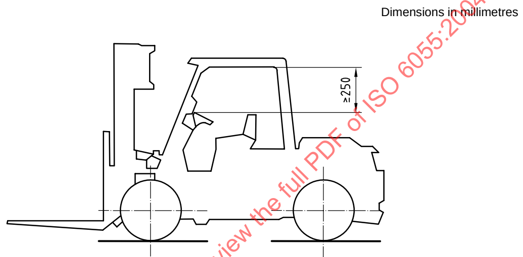
Figure 5 — Impact test permitted deformation — Seated operator truck
