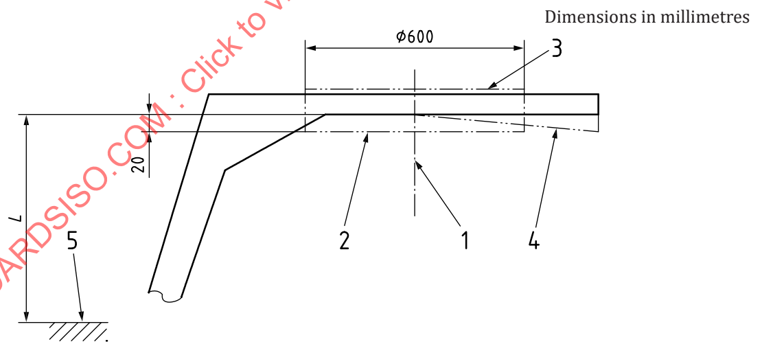
Figure 5 — Dynamic test permissible deformation — Overhead guard supported on all sides
