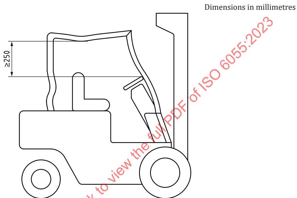
Figure 7 — Impact test permitted deformation — Sit-on truck
