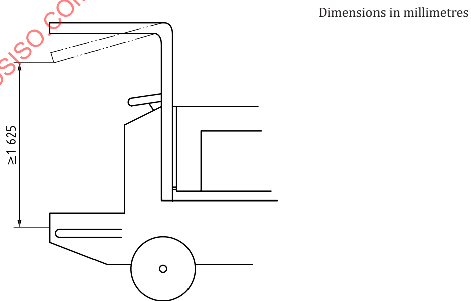
Figure 8 — Impact test permitted deformation — Stand-on truck
