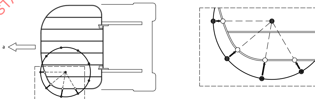
Figure 2 — Test object drop location points for sit-on truck above the SIP
