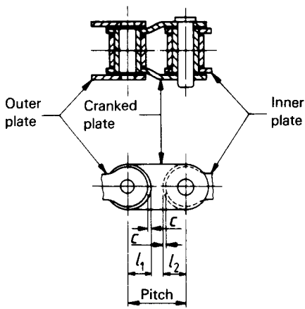
Cranked link
