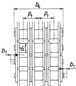
Triplex
