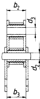
Plain pin
