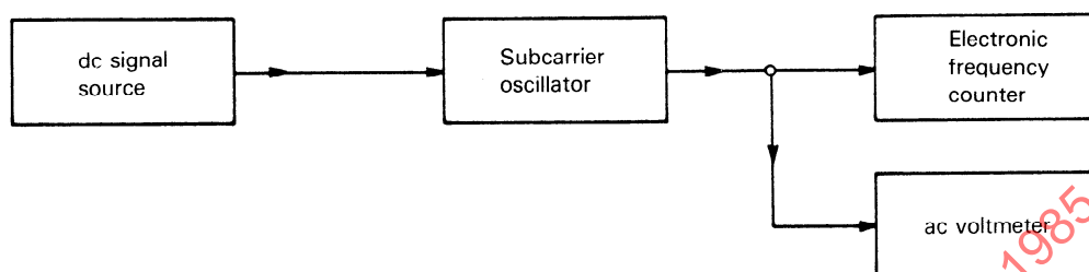
Figure 31 — Equipment configuration for amplitude modulation test
