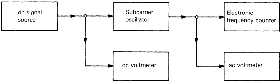
Figure 28 — Equipment configuration for control range(s) test(s)
