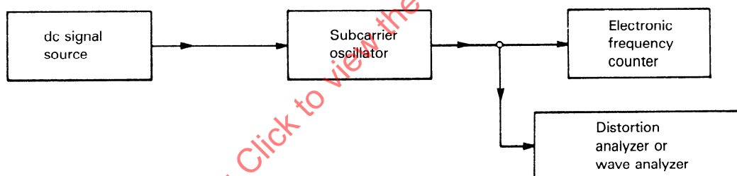
Figure 32 — Equipment configuration for output distortion test
