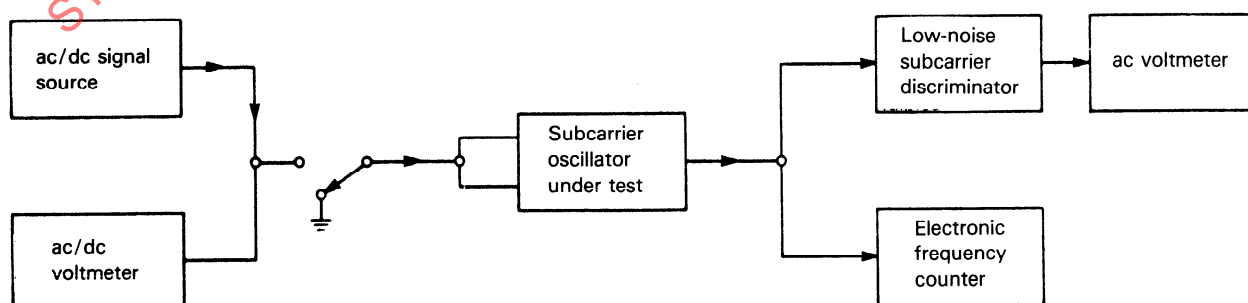
Figure 39 — Equipment configuration for common-mode rejection test
