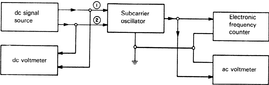
Figure 34 — Equipment configuration for input grounding test
