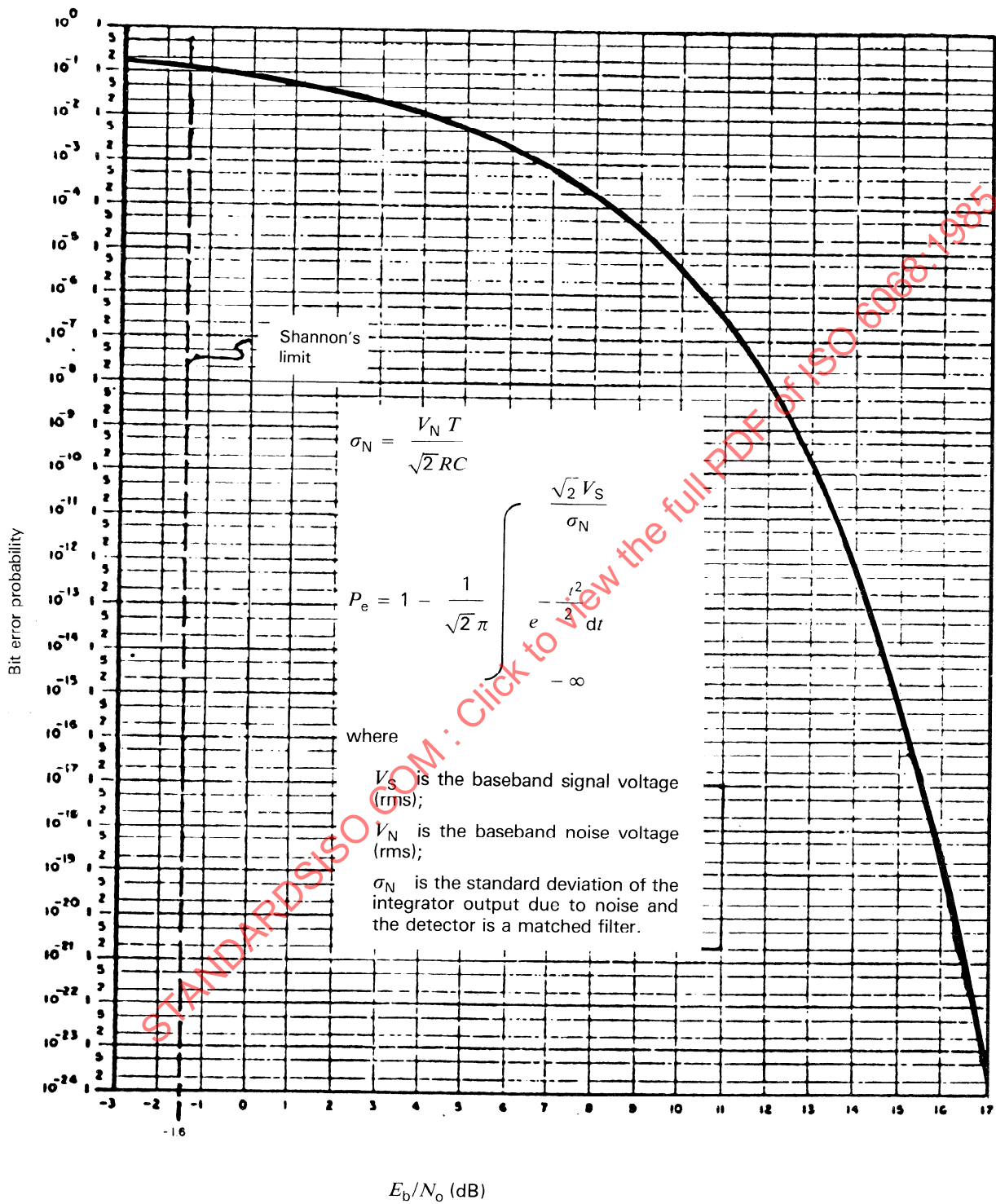
Figure 24 — Optimum theoretical performance for bit error rate versus normalized signal-to-noise ratio
