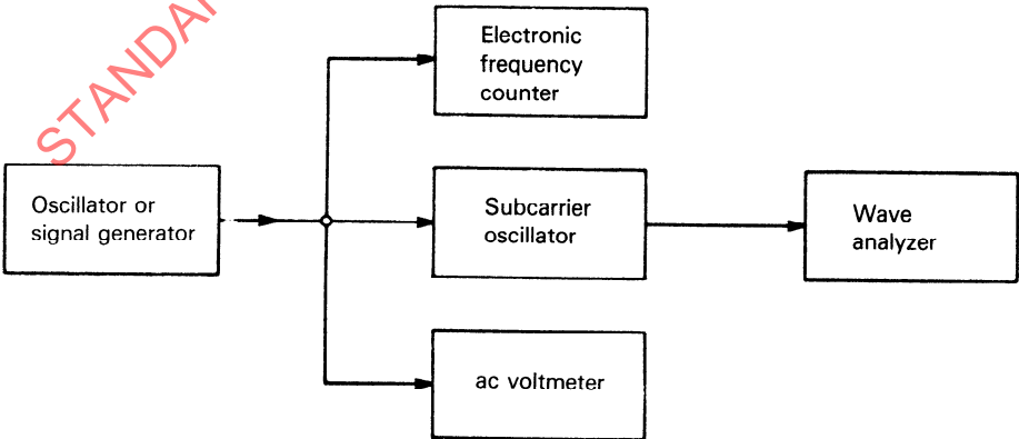
Figure 36 — Equipment configuration for modulation feedthrough test
