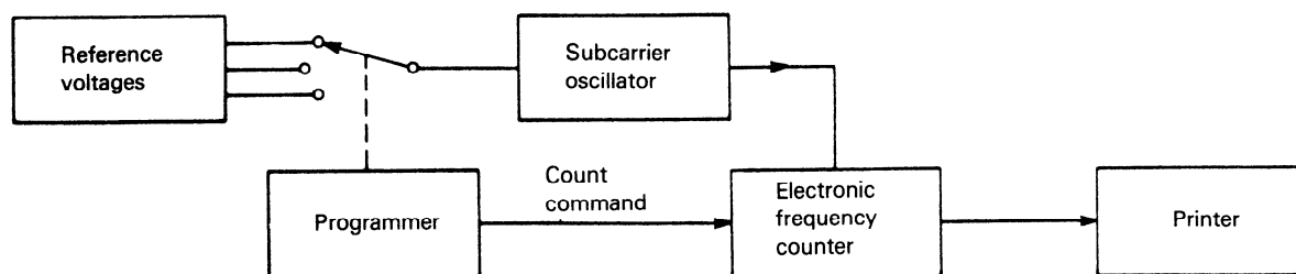
Figure 37 — Equipment configuration for stability versus time test
