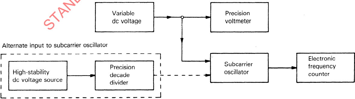
Figure 30 — Equipment configuration for linearity measurement, method no. 2
