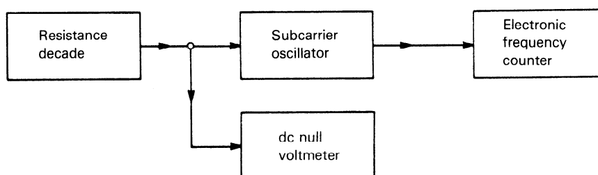
Figure 33 — Equipment configuration for source impedance test
