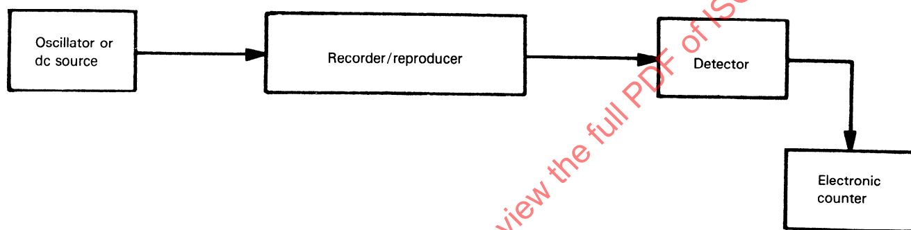
Figure 10 — Tape speed — Method I
