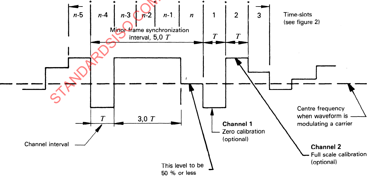
Figure 7 — One-hundred percent duty factor PAM with amplitude synchronization
