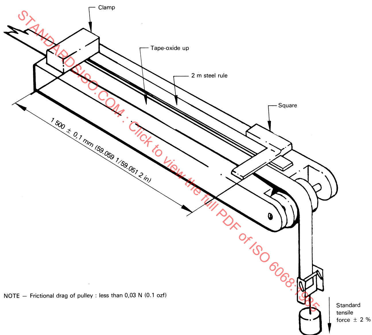
Figure 9 — Speed test-tape preparation
