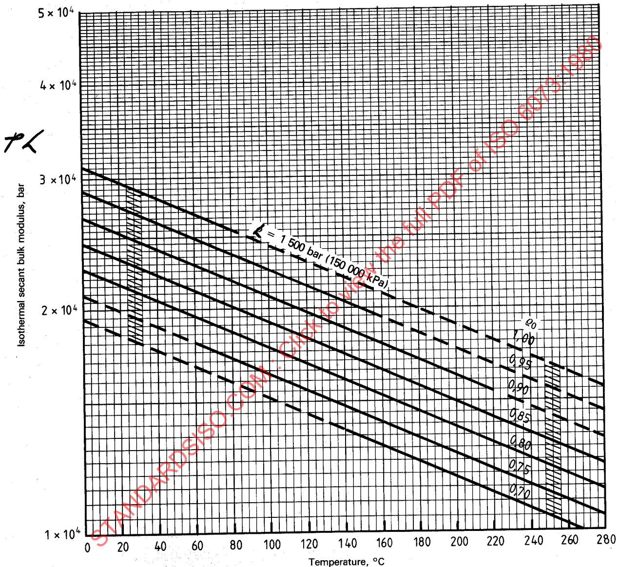
Figure 1 — Secant bulk modulus at 1 500 bar (150 000 kPa) gauge pressure versus temperature and density for petroleum oils
