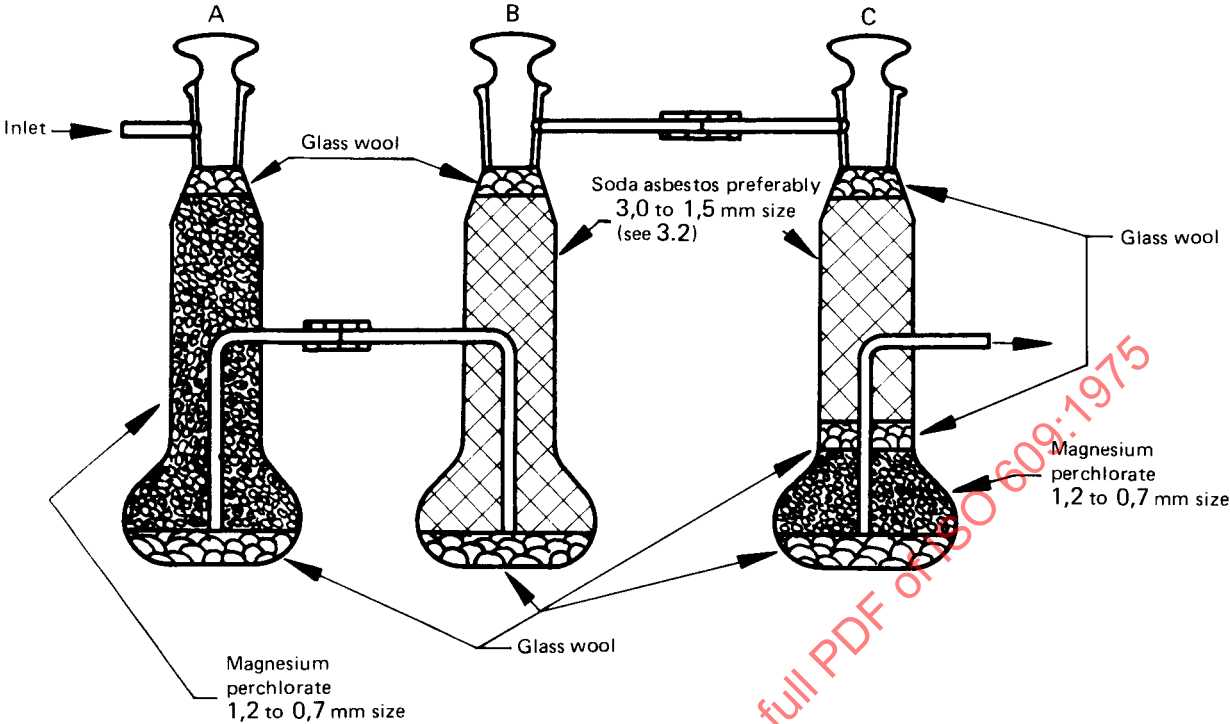
FIGURE 3 – Absorption train
