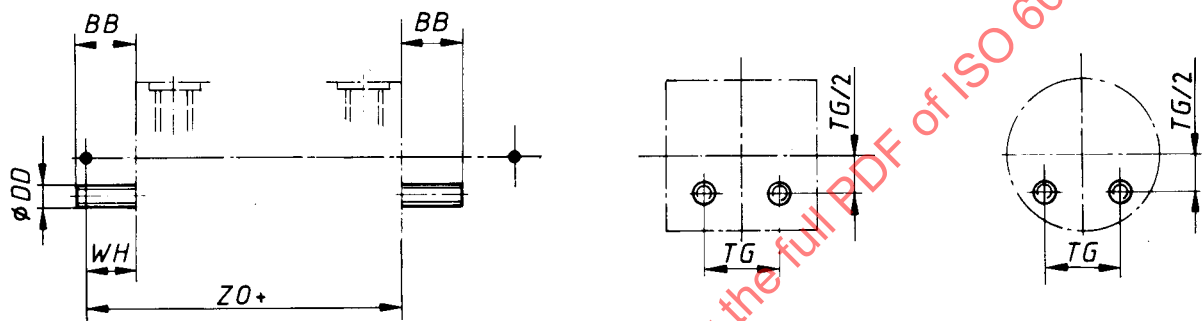
Figure 51 — (MDX 4) Both ends 2 studs or tie rods extended — Double rod
