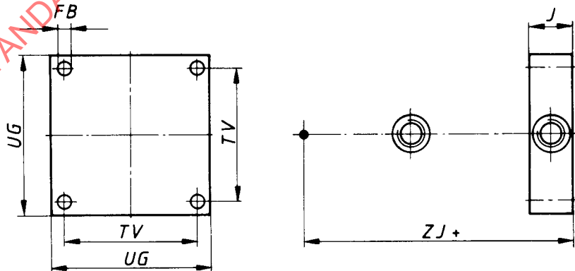
Figure 12 — (ME 10) Cap, square
