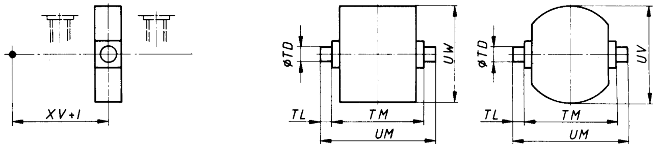
Figure 41 — (MT 4) Intermediate fixed or movable trunnion (male)
