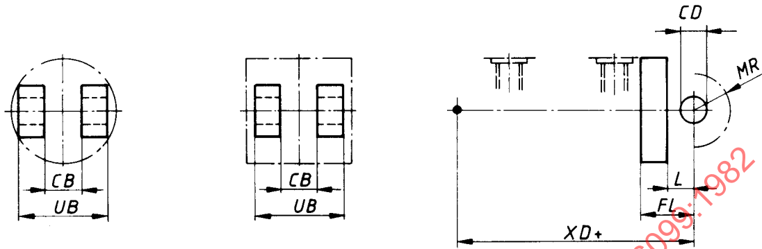
Figure 25 — (MP 2) Cap detachable clevis
