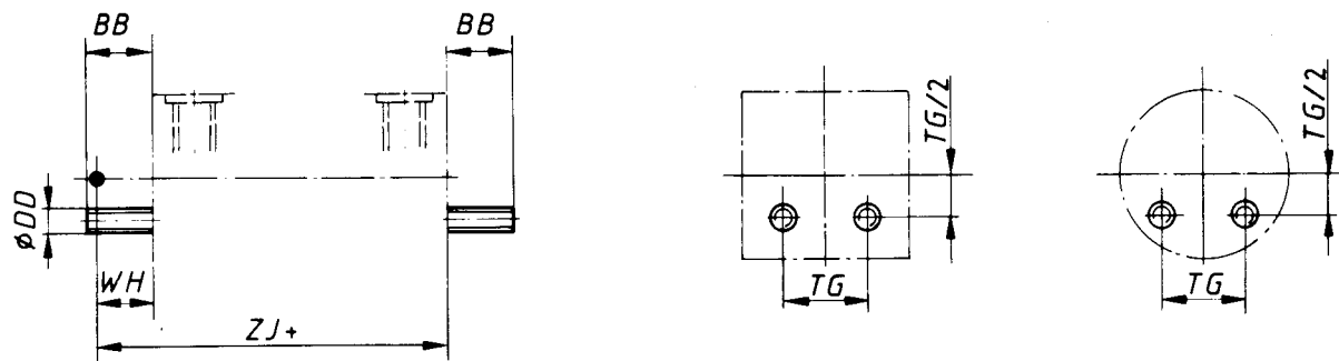
Figure 50 — (MX 4) Both ends 2 studs or tie rods extended
