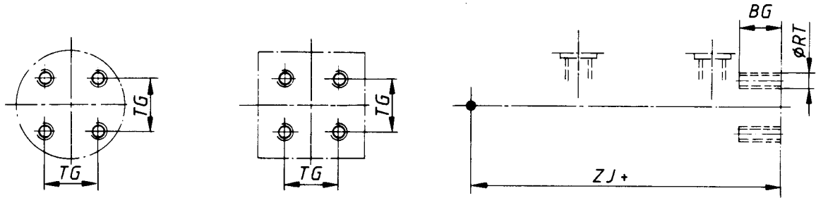
Figure 54 — (MX 6) Cap, tapped
