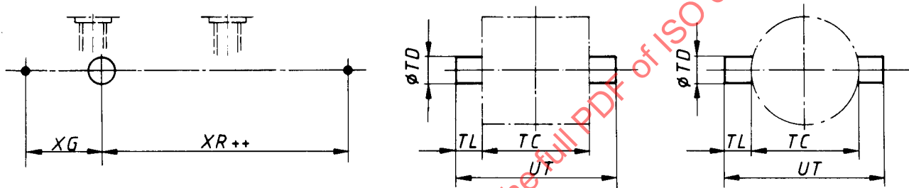
Figure 39 — (MDT 1) Head, integral trunnion (male) — Double rod
