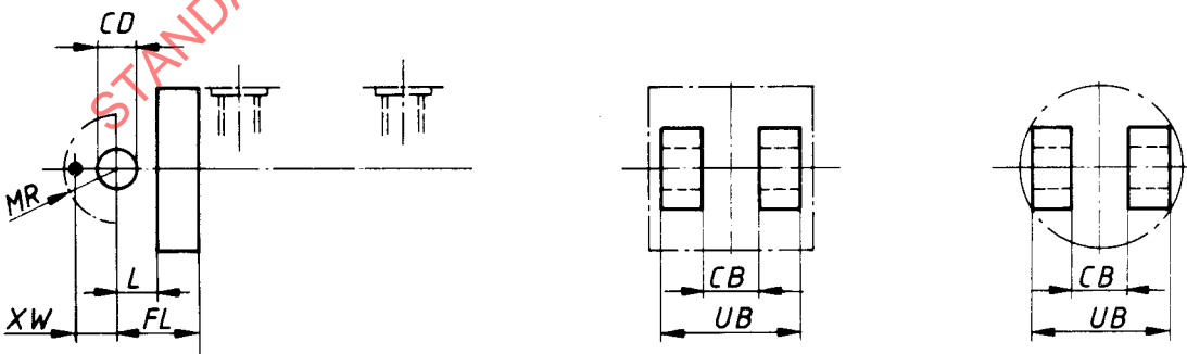
Figure 30 — (MP 7) Head detachable clevis
