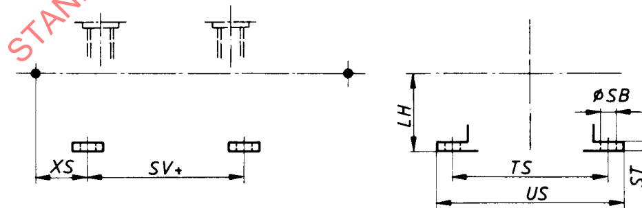
Figure 37 — (MDS 2) Side lugs — Double rod
