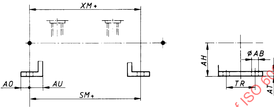
Figure 35 — (MDS 1) End angles — Double rod
