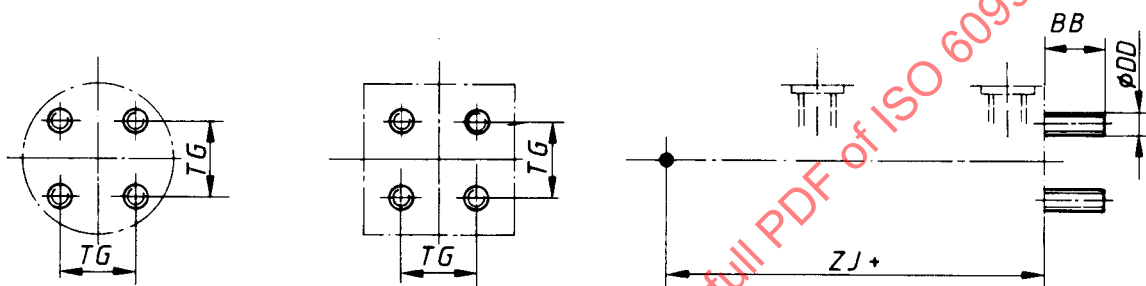
Figure 47 — (MX 2) Cap studs or tie rods extended
