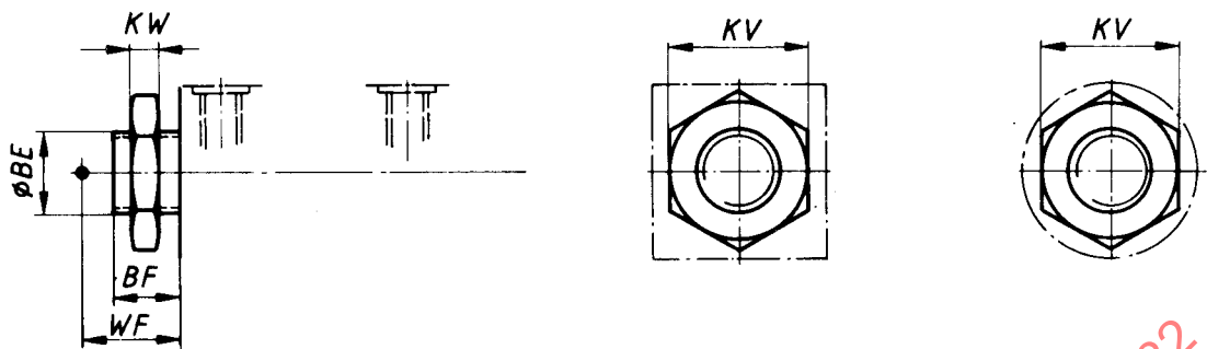
Figure 31 — (MR 3) Head, threaded
