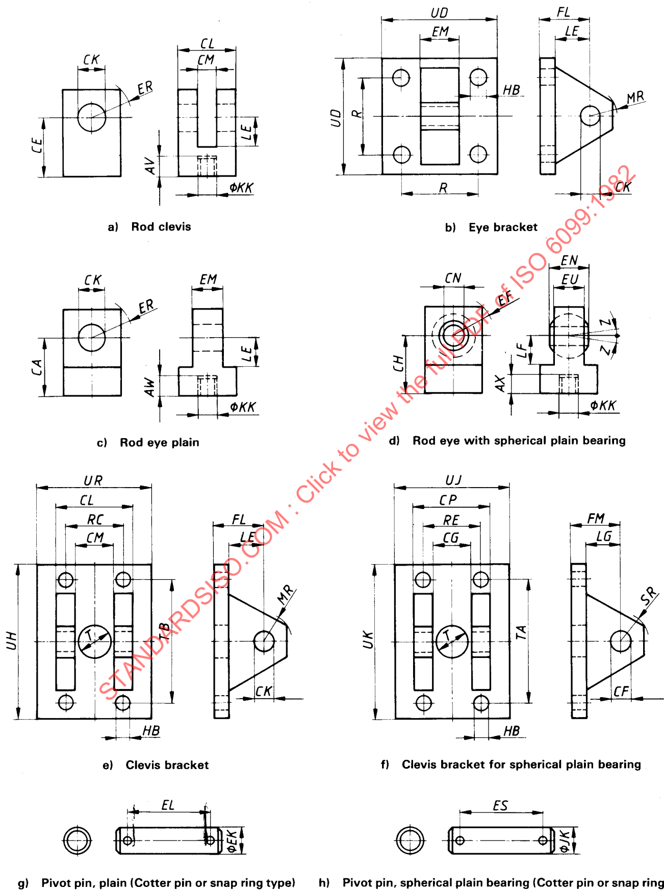
Figure 3 — Cylinder accessories
