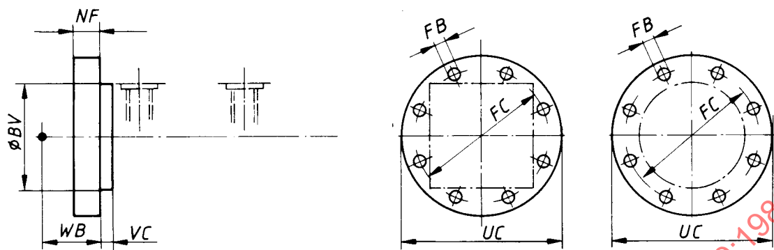
Figure 22 — (MF 7) Head circular flange centred on the rearside
