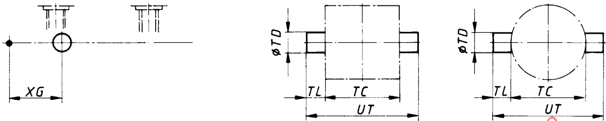
Figure 38 — (MT 1) Head integral trunnion (male)
