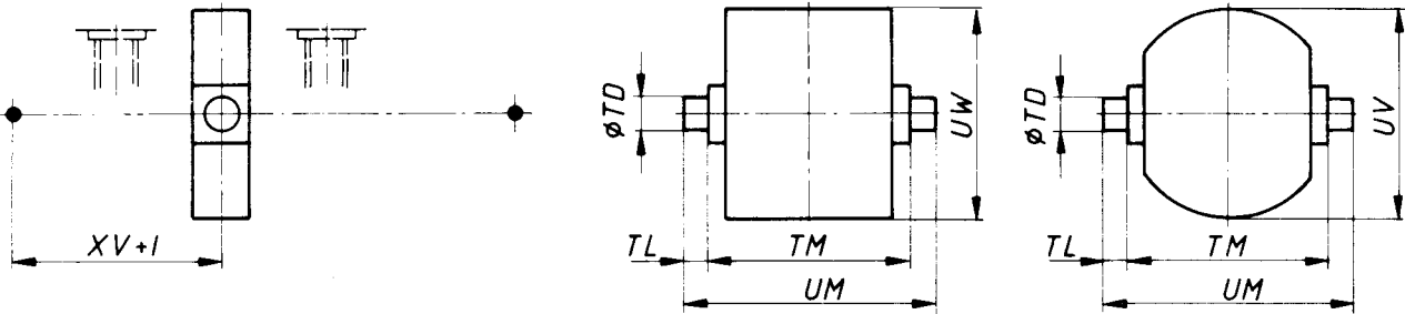
Figure 42 — (MDT 4) Intermediate fixed or movable trunnion (male) — Double rod
