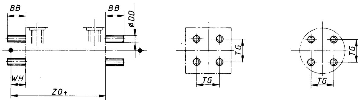
Figure 46 — (MDX 1) Both ends studs or tie rods extended — Double rod
