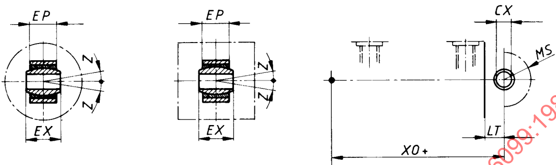
Figure 28 — (MP 5) Cap fixed eye with spherical plain bearing
