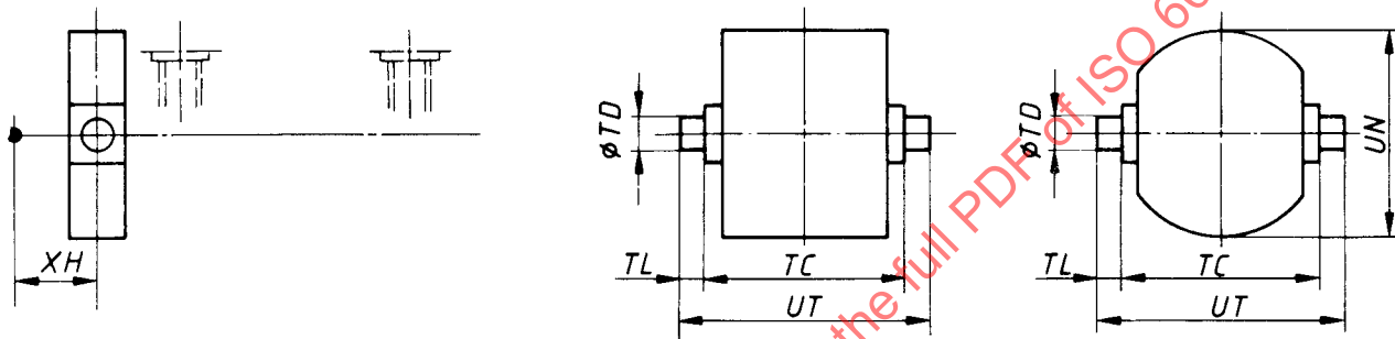
Figure 43 — (MT 5) Head detachable trunnion (male)
