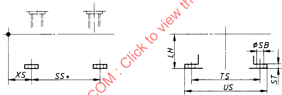
Figure 36 — (MS 2) Side lugs
