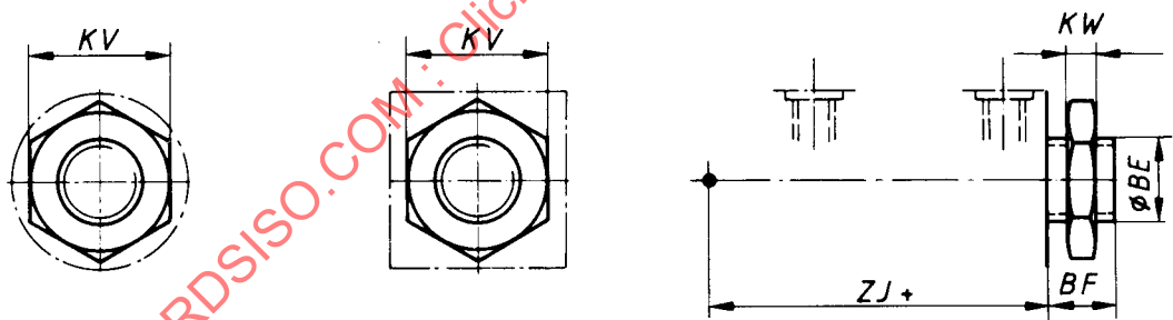
Figure 33 — (MR 4) Cap, threaded
