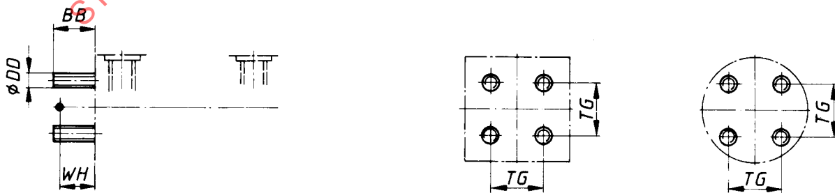
Figure 49 — (MX 3) Head studs or tie rods extended
