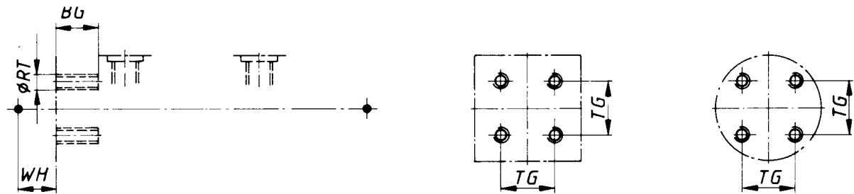
Figure 53 — (MDX 5) Head, tapped — Double rod
