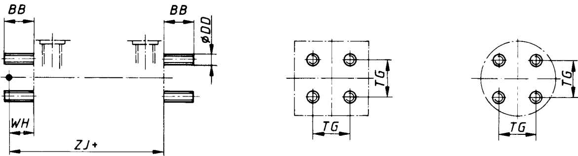
Figure 45 — (MX 1) Both ends studs or tie rods extended
