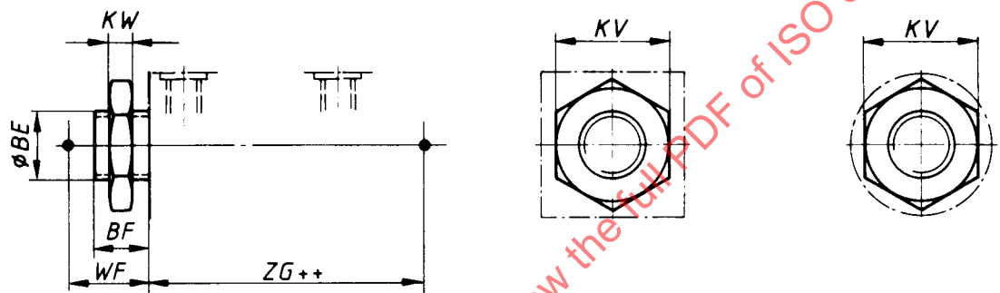
Figure 32 — (MDR 3) Head, threaded — Double rod
