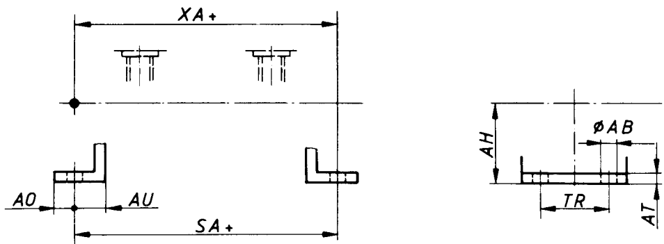
Figure 34 — (MS 1) End angles
