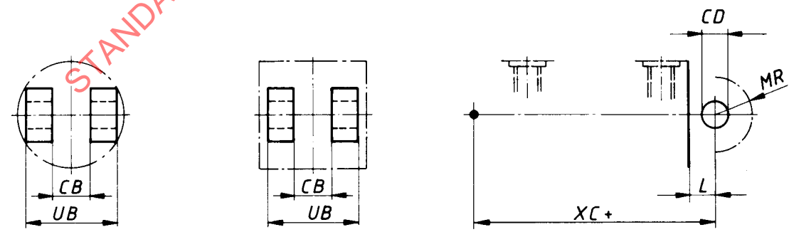
Figure 24 — (MP 1) Cap fixed clevis
