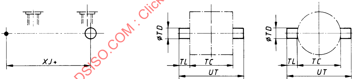
Figure 40 — (MT 2) Cap integral trunnion (male)
