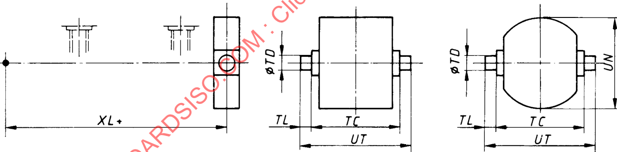
Figure 44 — (MT 6) Cap detachable trunnion (male)
