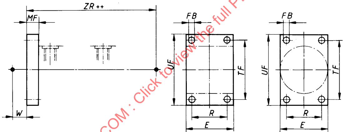
Figure 14 — (MDF 1) Head, rectangular flange — Double rod
