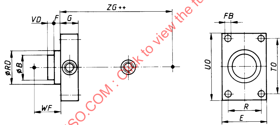
Figure 5 – (MDE 5) Head, rectangular — Double rod
