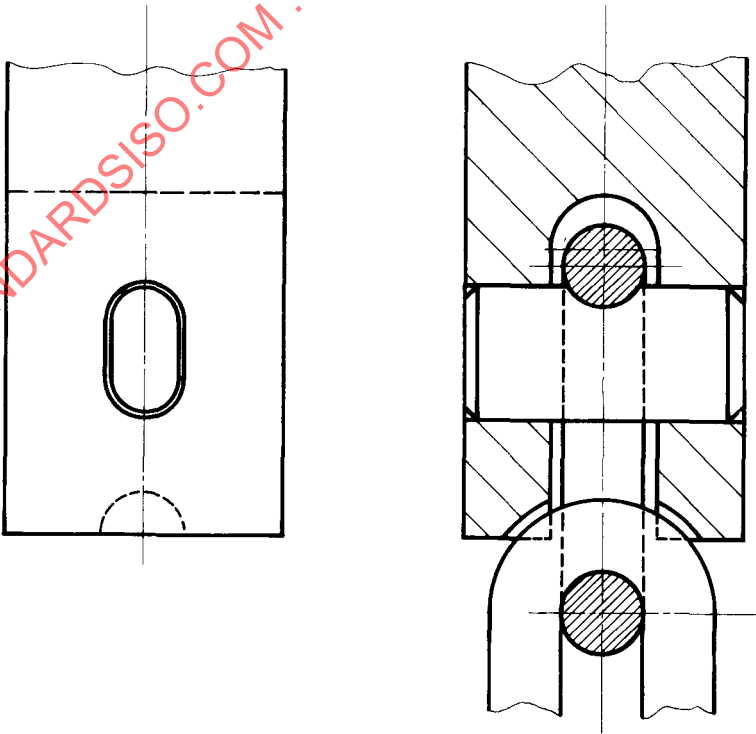
FIGURE 5 – Anchorage fork
