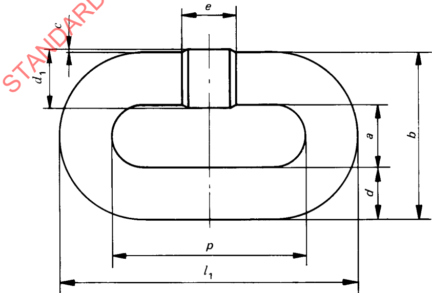
FIGURE 2 — Chain link dimensions
