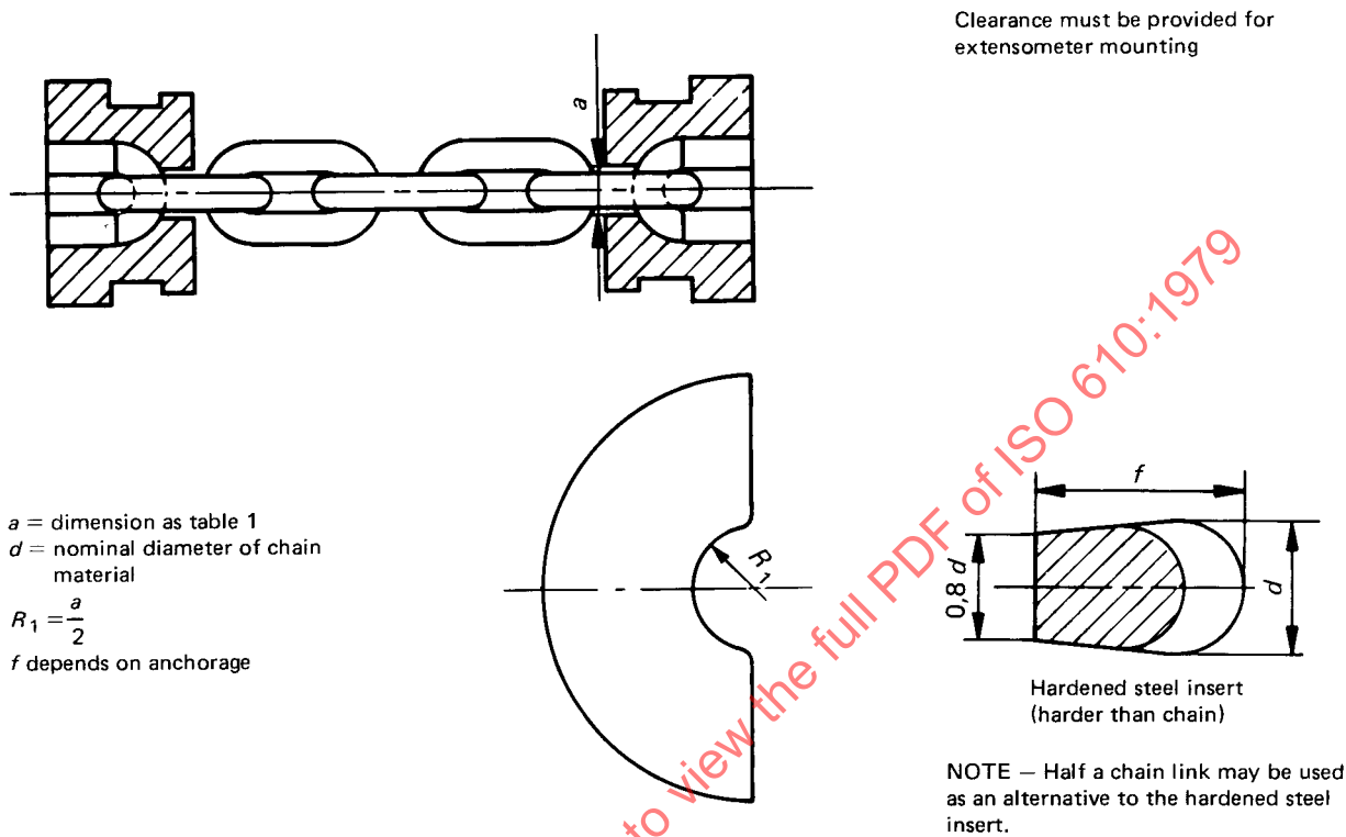
FIGURE 3 — Chain anchorage for static tensile test
