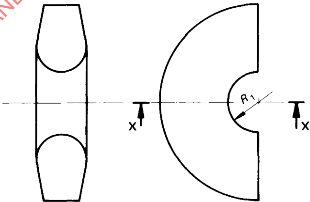
FIGURE 3 — Chain anchorage for static tensile test
