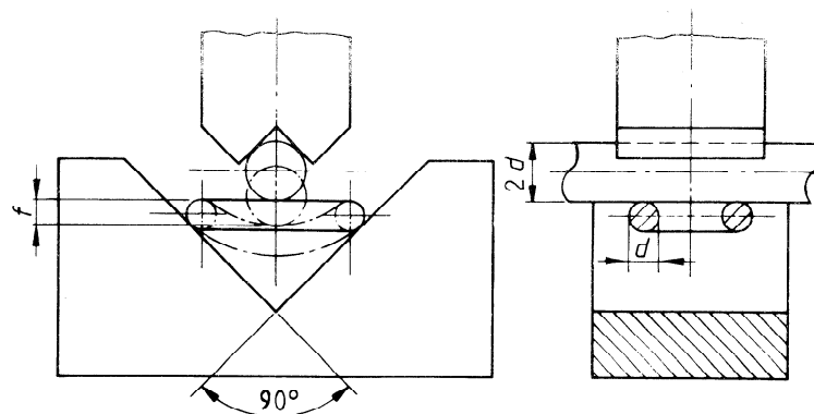
Figure 6 — Bend test
