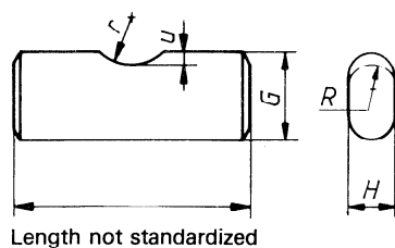
Figure 4 — Anchorage pin
