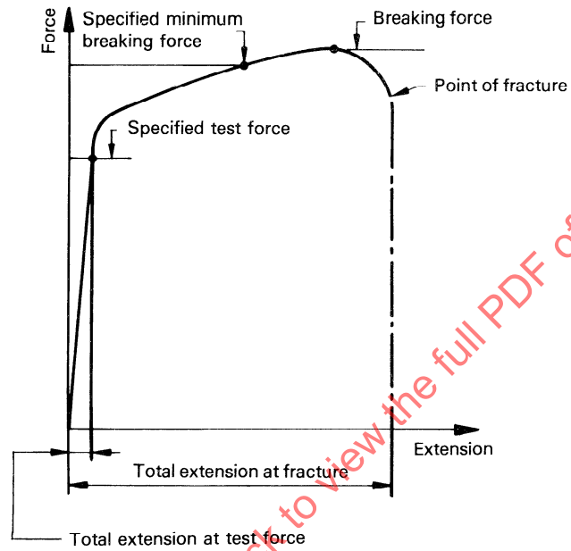
Figure A.1 — Force-extension diagram — Illustration of terms
