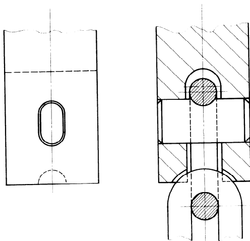
Figure 5 — Anchorage fork
