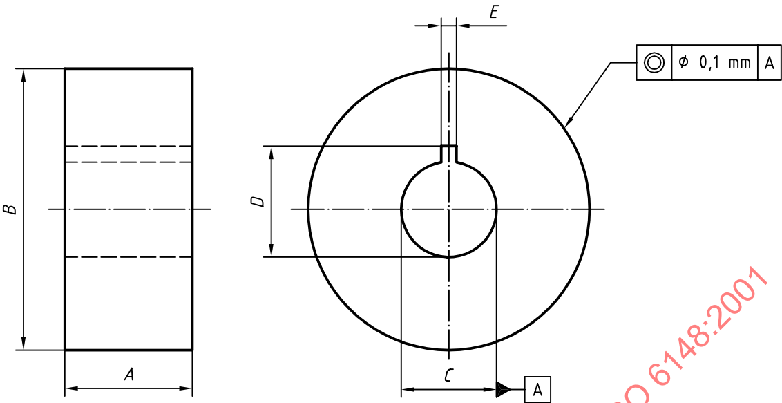
Figure 3 — Core dimensions
