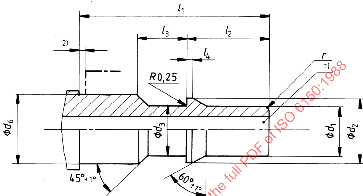
Figure 3 — Plug for 25 bar (2,5 MPa) maximum working pressure (series C)
