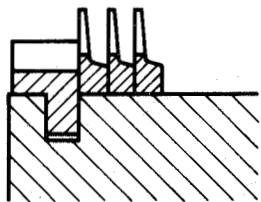
Figure 9 — Application of L type wire on roller
