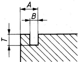
Figure 8 — Groove for L type wire
