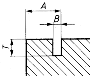
Figure 5 — Groove for I type wire
