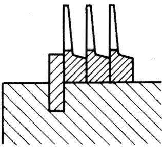
Figure 6 — Application of I type wire on roller
