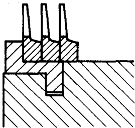
Figure 3 — Application of Z type wire on roller
