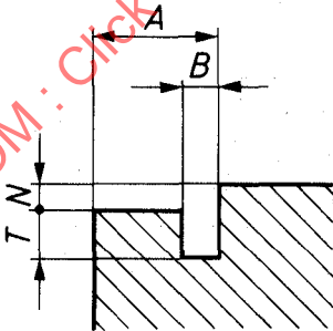
Figure 2 — Groove for Z type wire
