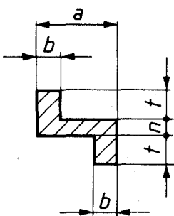
Figure 1 — Section of Z type wire
