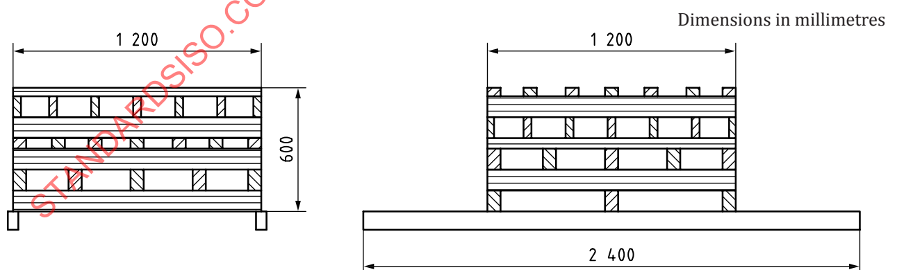
Figure 18 — Test crib
