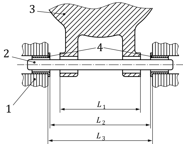
c) Total axial clearance, C_{TA} = L_2 - L_1 ; Bushing projection = (L_3 - L_2)/2
