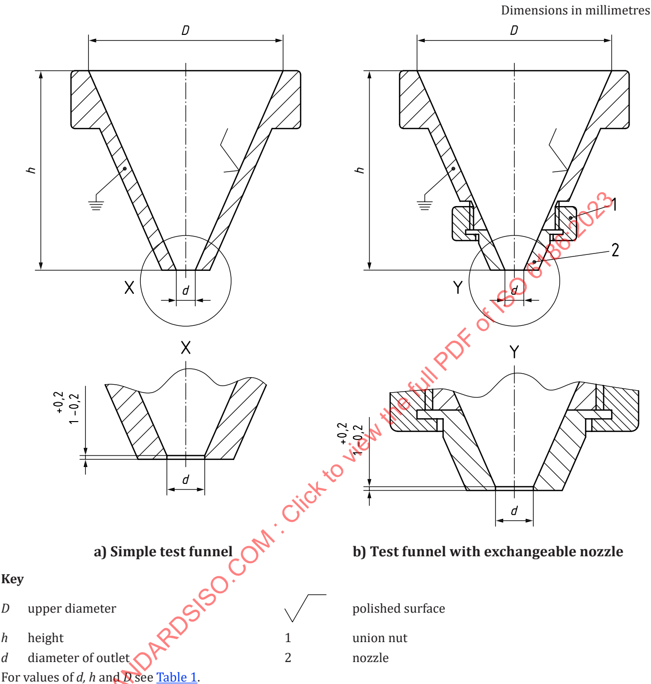
Figure 1 — Test funnel
