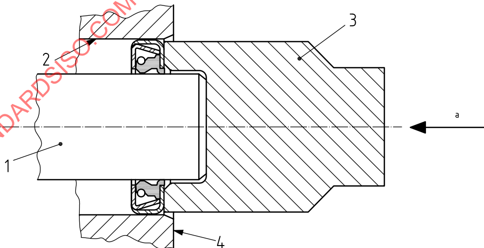
Figure 2 — Installation of seal — Bottom bore (seal bottoms on machined bore shoulder)
