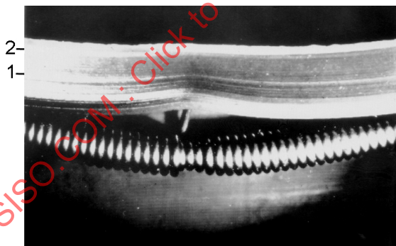
Figure 23 — Spring with incomplete joint portion
