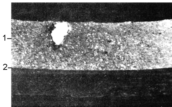
Figure 4 — Inclusion: filler
