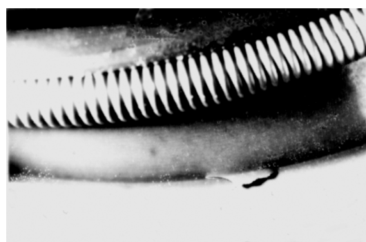
Figure 18 — Crack
