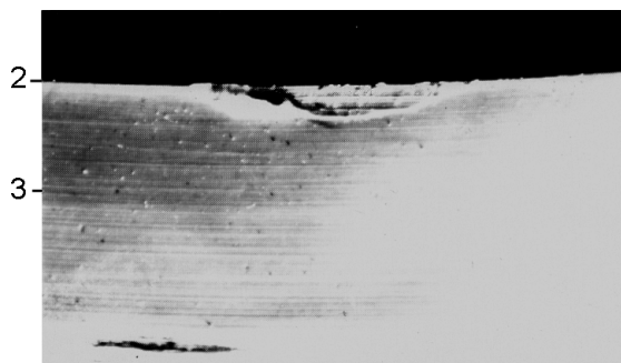
Figure 14 — Stuck flash
