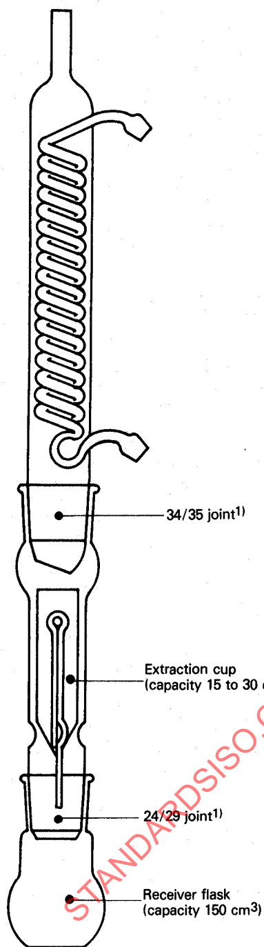
Figure 1 — Type 1 extraction apparatus
