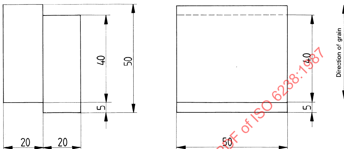
Figure 2 — Form and dimensions of test specimen
