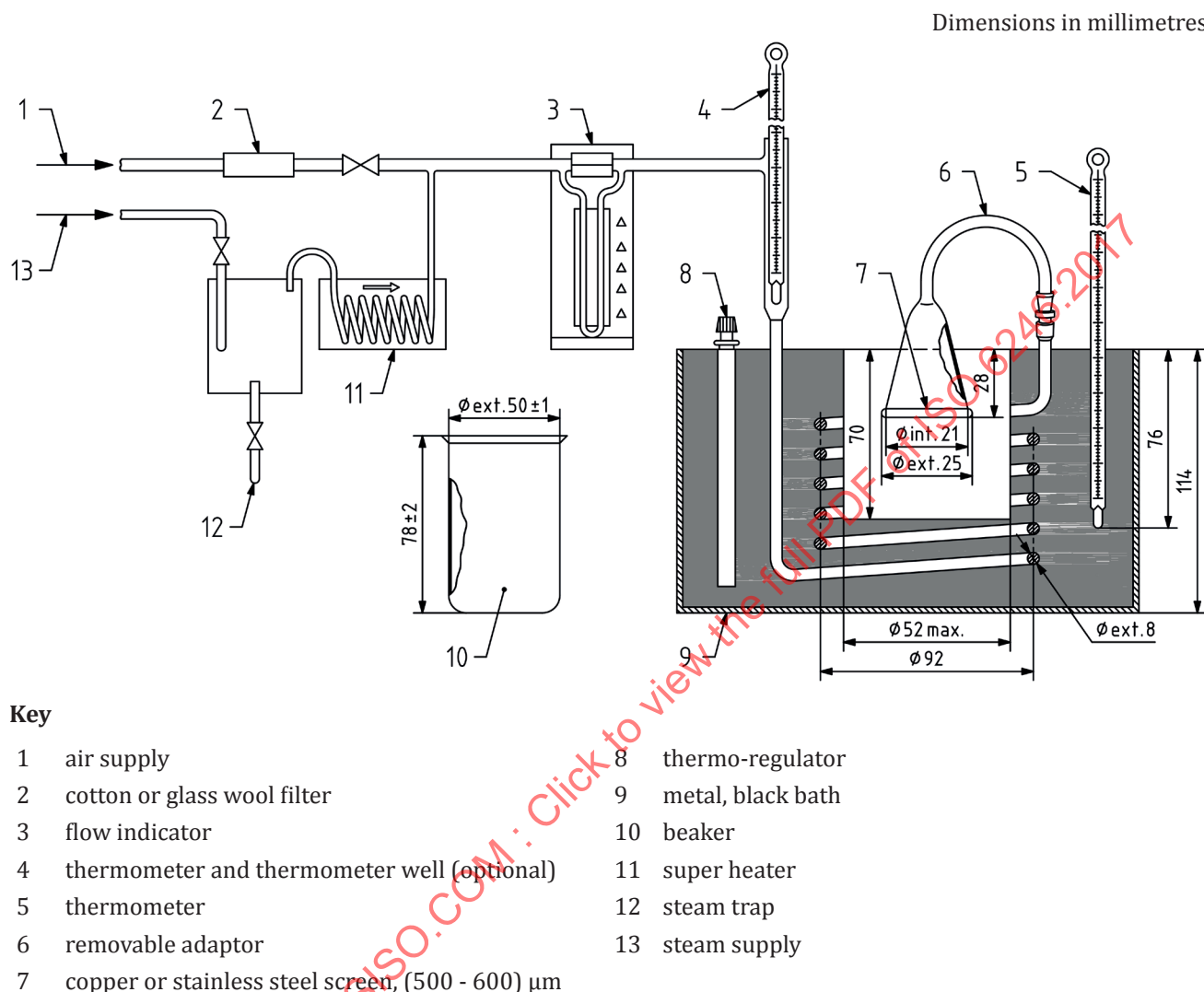
Figure 1 — Apparatus for determining gum content by jet evaporation
