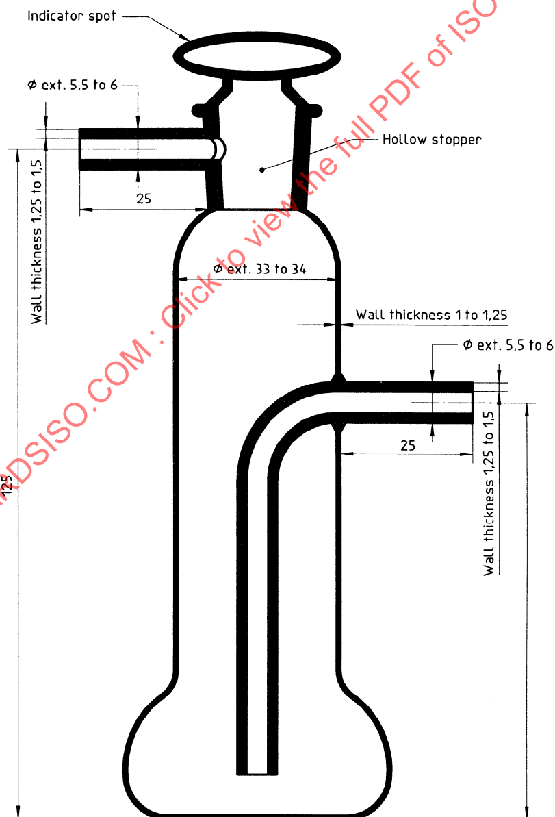
Figure 1 — Midvale tube
