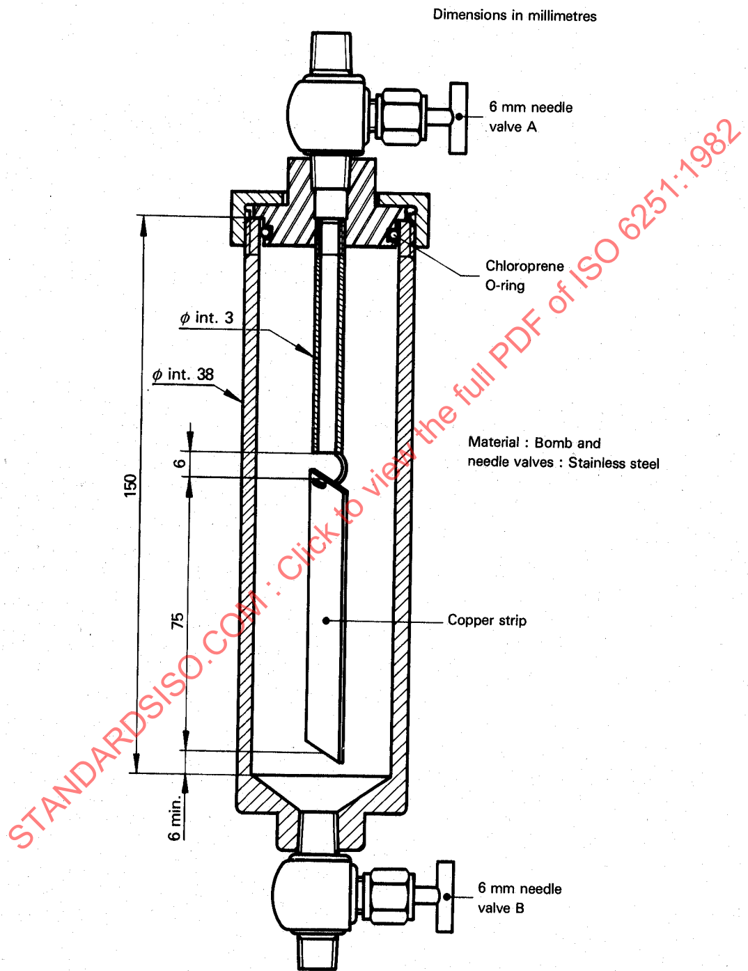
Figure — Copper strip corrosion test cylinder
