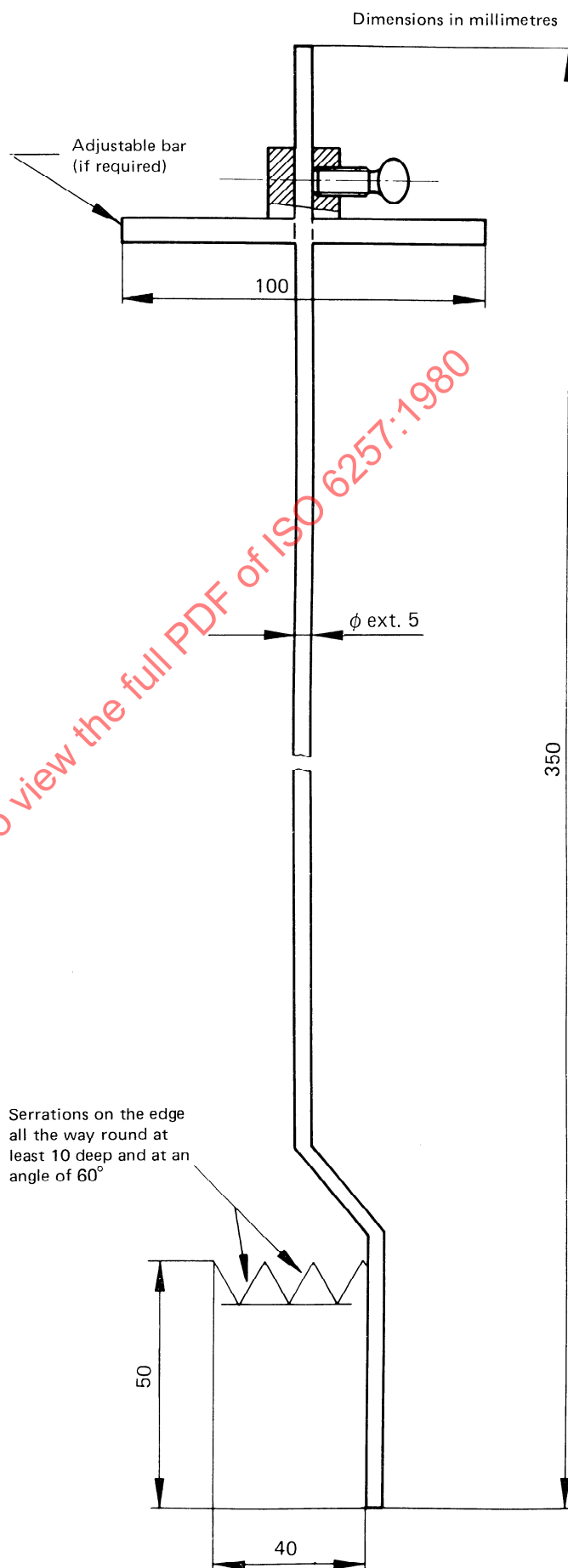
Figure 10 — Typical ladle
