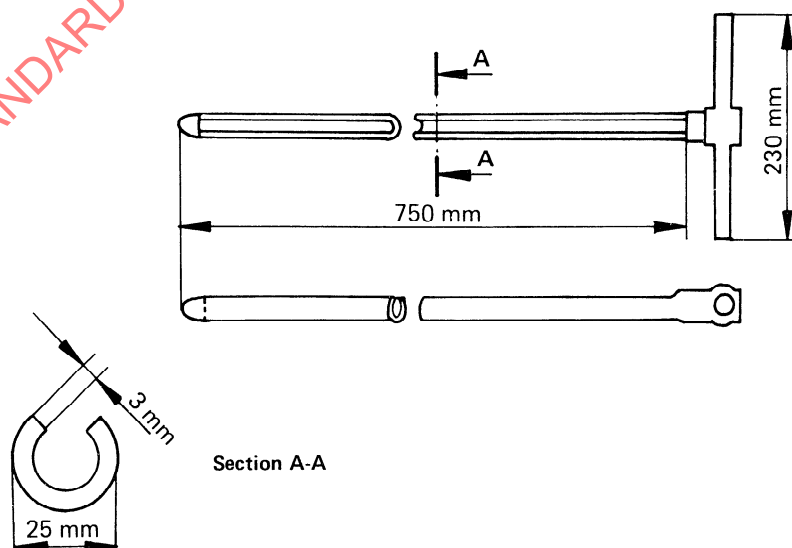
Figure 3 — Closed-end sampling spear — Typical dimensions
