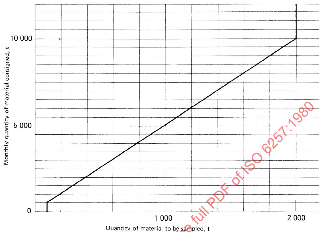
Figure 4 — Quantity of material to be sampled as a function of the monthly quantity of material consigned
