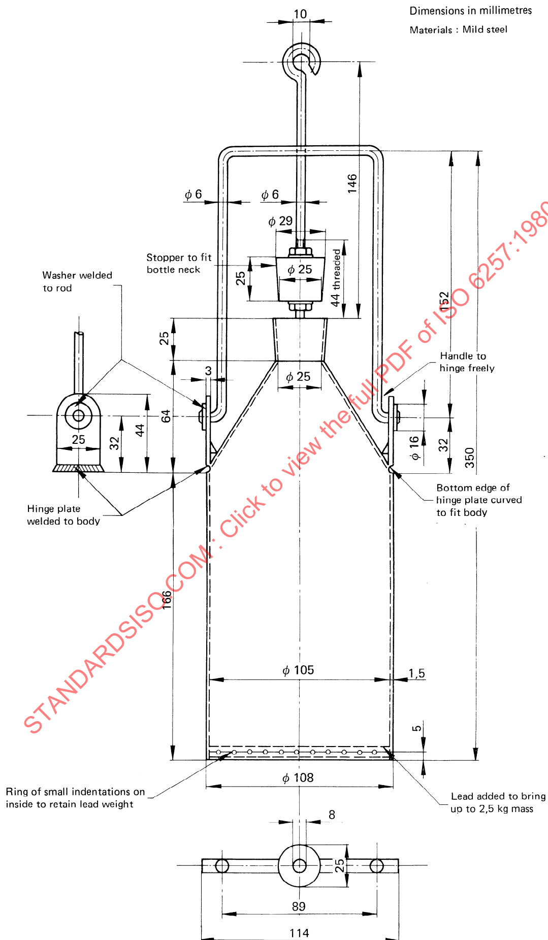
Figure 8 — Typical weighted sampling can
