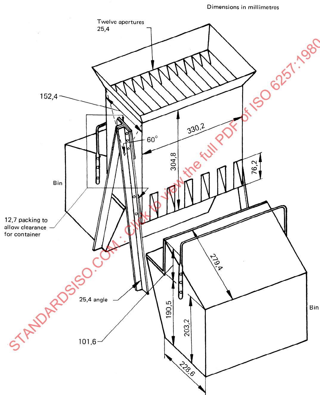
Figure 11 — Typical riffle for sample size reduction of material with particle size of approximate diameter 5 mm
