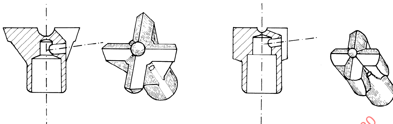
Figure 1 — Typical cutting bits for sampling drill
