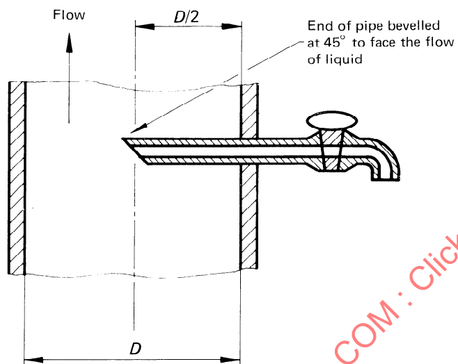
Figure 9 — Typical pipeline sampler
