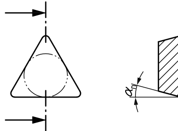
Figure 1 — Normal clearance, \alpha_n
