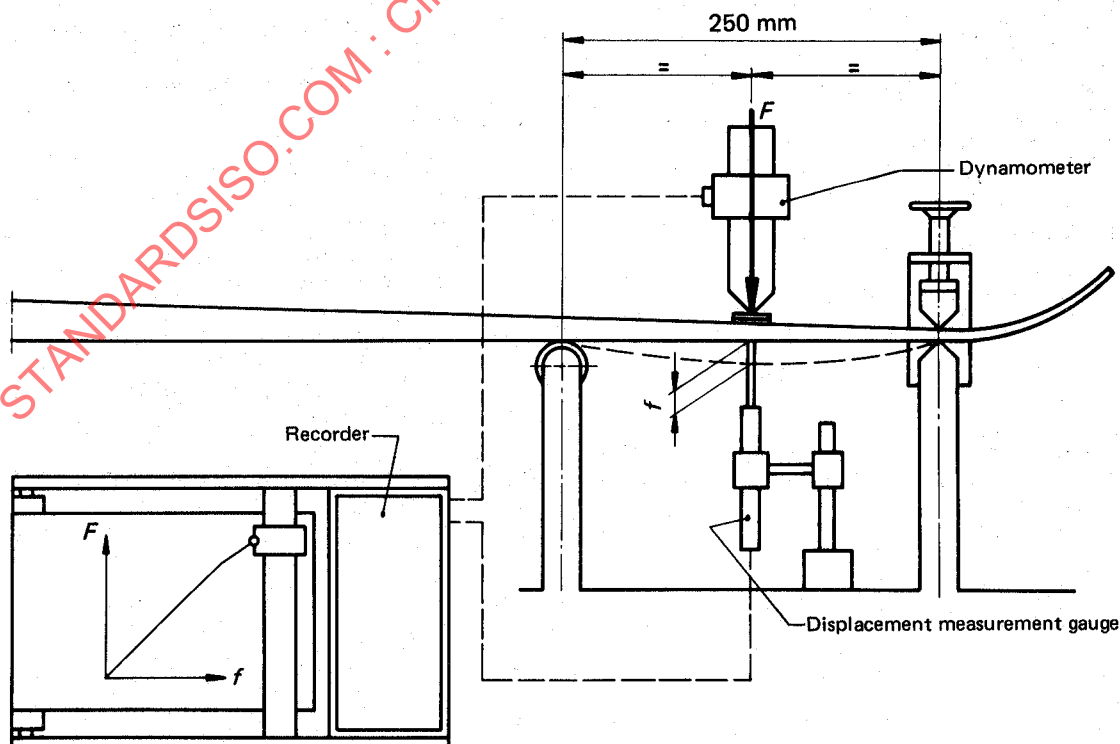
Figure 1 — Testing machine
