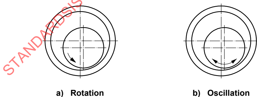
Figure 2 — Rotational motion of journal
