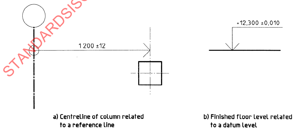
Figure 2 — Examples of limit deviations for position dimensions
