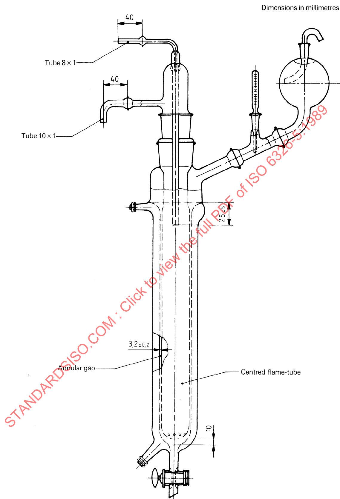
Figure 2 — Combustion vessel
