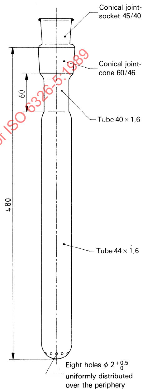
Figure 4 — Flame tube
