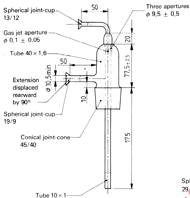
Figure 5 — Burner
