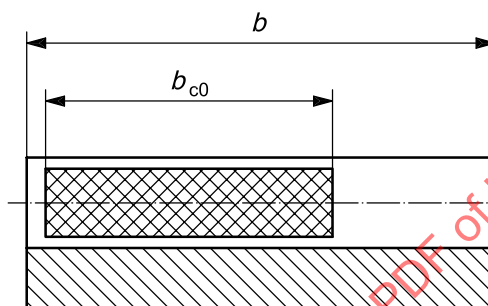
Figure A.1 — Length of contact pattern b_{c0} and face width b
