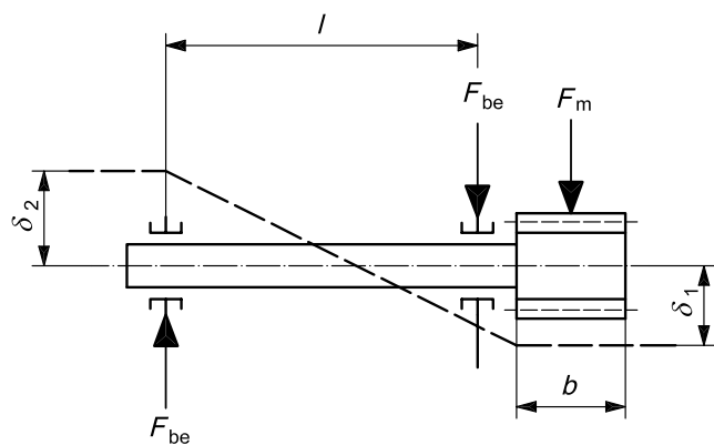
Figure 15 — Loading and deflections for overhung gear [see Equation (68)]
