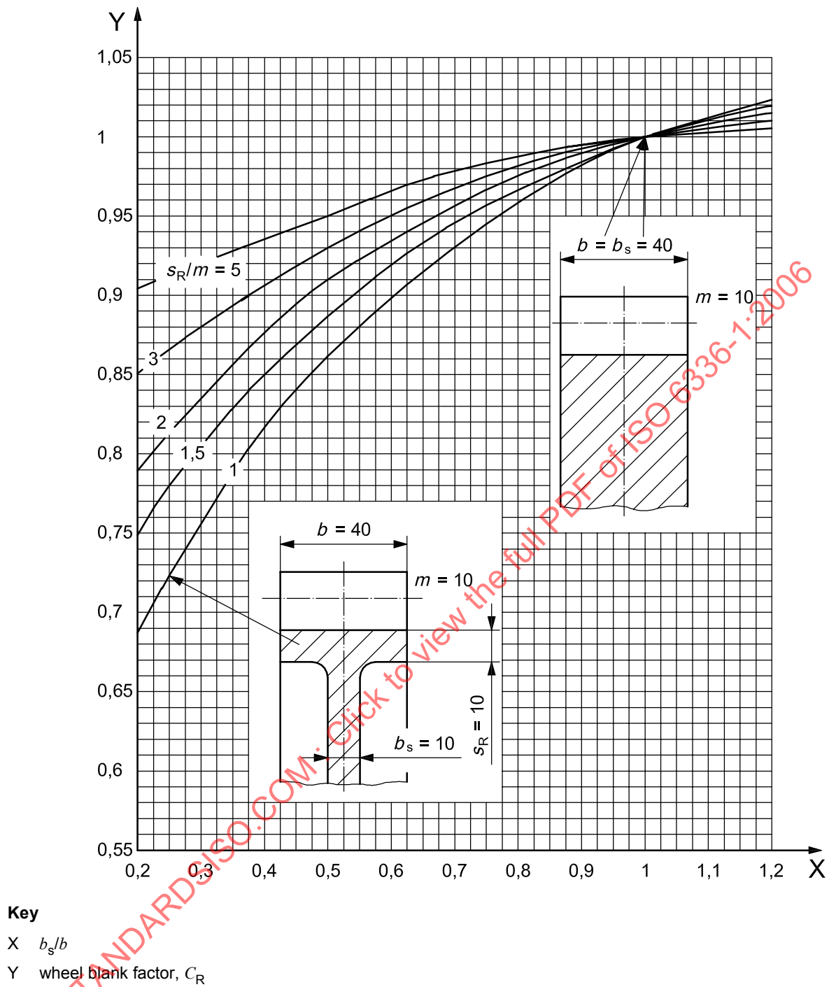
Figure 19 — Wheel blank factor C_R — Mean values for mating gears of similar or stiffer wheel blank design
