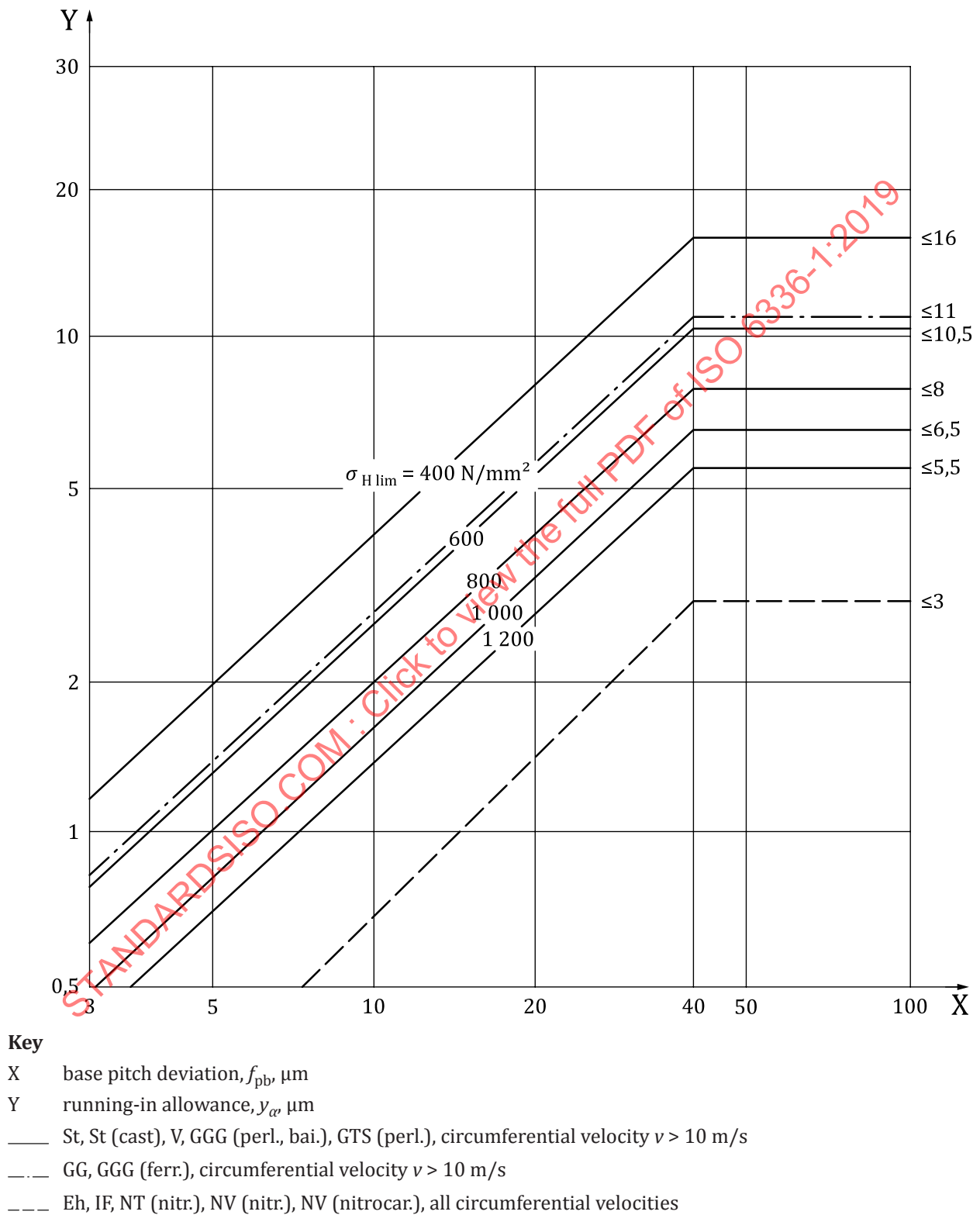
Figure 17 — Determination of running-in allowance, y_\alpha , of gear pair (see also Figure 18 )
