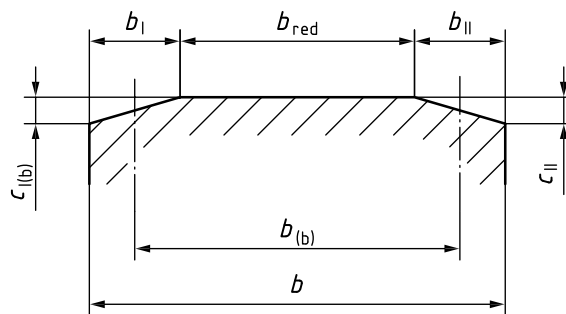
Figure B.2 — Amount, C_{I(II)-(b)} , and width, b_{(b)} , of end relief (see 7.5.3.5)
