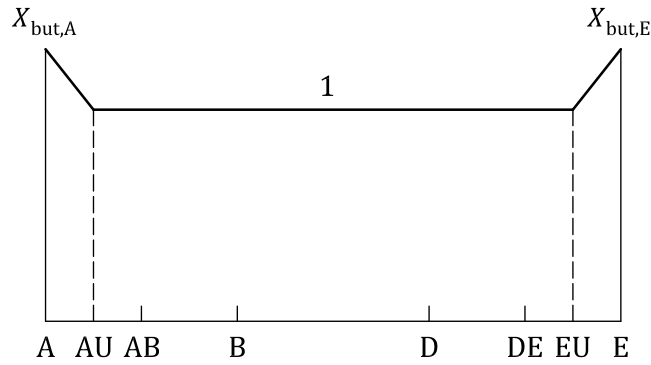
Figure 26 — Buttressing factor, X_{but,CP}
