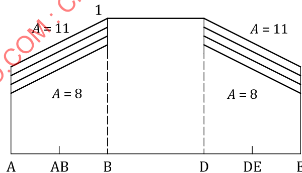
Figure 22 — Load sharing factor for cylindrical gears with unmodified profiles and tolerance class 8
