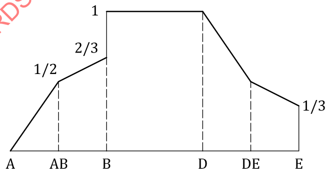
Figure 24 — Load sharing factor for cylindrical spur gears with adequate profile modification on the addendum of the wheel and/or the dedendum of the pinion
