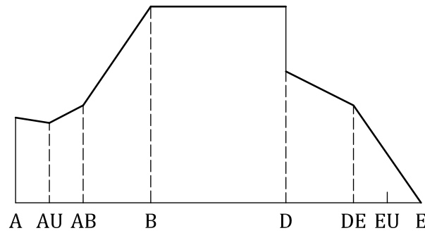
Figure 30 — Load sharing factor for cylindrical helical gears with \varepsilon_\beta \leq 0,8 and adequate profile modification on the addendum of the pinion and/or the dedendum of the wheel
