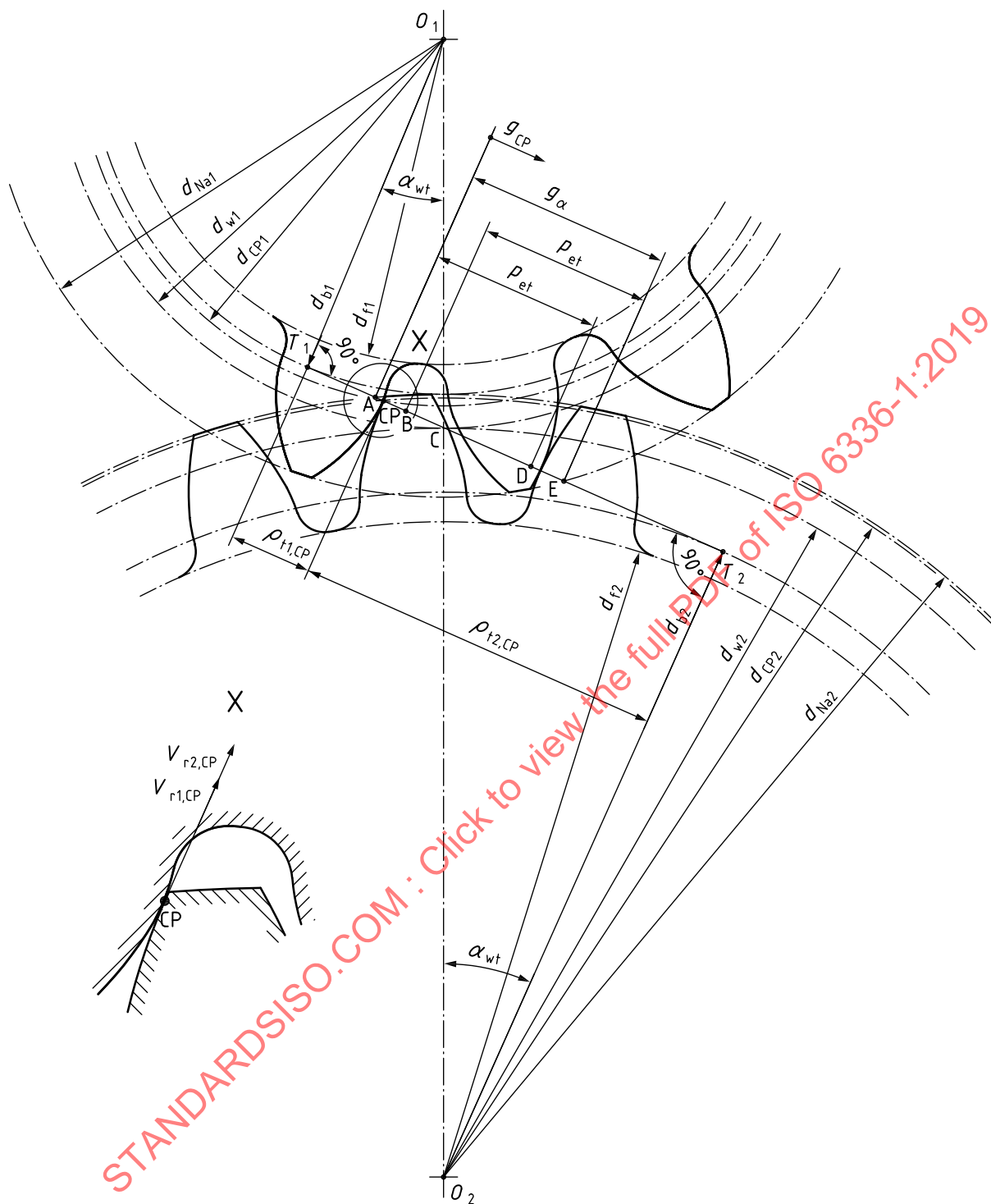
Figure 20 — Definition of contact point CP on the line of action
