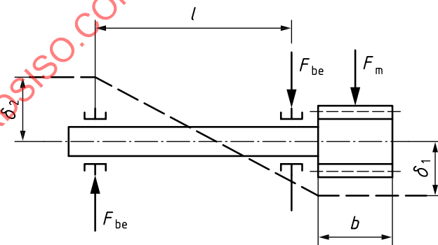
Figure 15 — Loading and deflections for overhung gear [see Formula (70) ]
