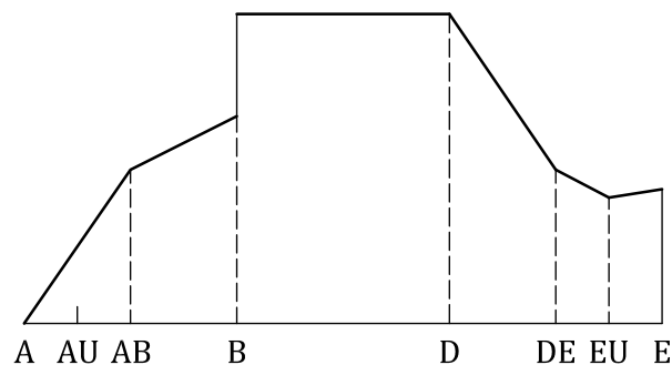
Figure 29 — Load sharing factor for cylindrical helical gears with \varepsilon_\beta \leq 0,8 and adequate profile modification on addendum of the wheel and/or the dedendum of the pinion
