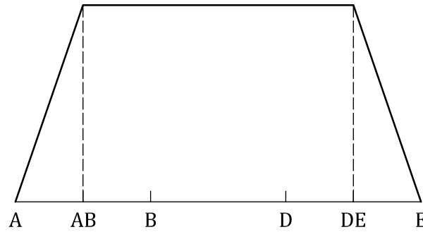
Figure 32 — Load sharing factor for cylindrical helical gears with \varepsilon_\beta \geq 1,2 and adequate profile modification
