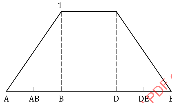
Figure 23 — Load sharing factor for cylindrical spur gears with adequate profile modification
