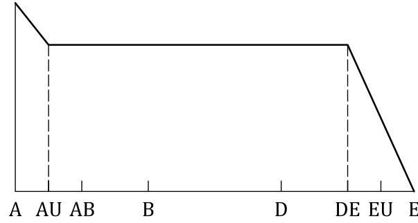
Figure 34 — Load sharing factor for cylindrical helical gears with \varepsilon_\beta \geq 1,2 and adequate profile modification on the addendum of the pinion and/or dedendum of the wheel
