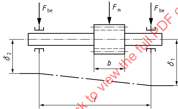
Figure 14 — Loading and deflections for gear mounted between the bearings [see Formula (69) ]
