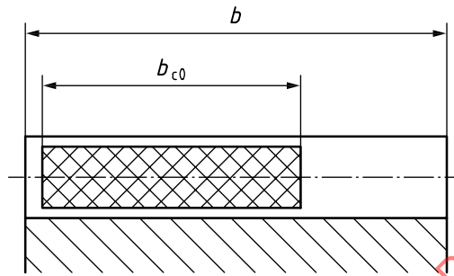
Figure A.1 — Length of contact pattern b_{\text{c0}} and face width b
