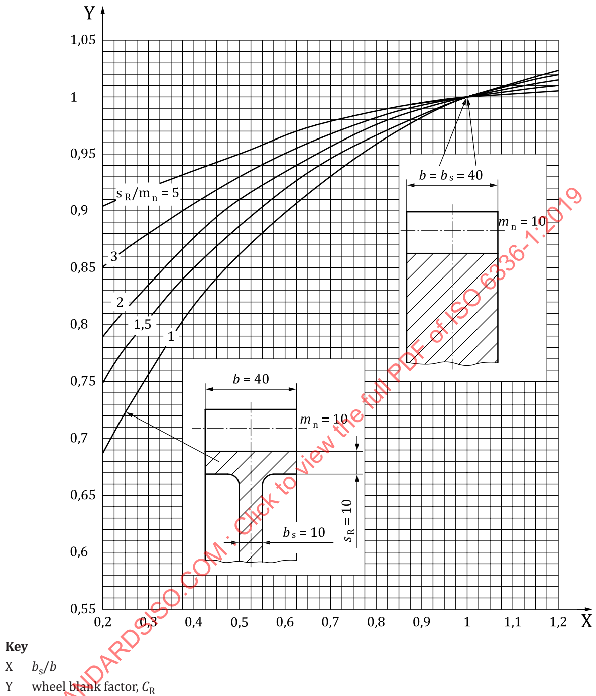
Figure 19 — Gear blank factor, C_R — Mean values for mating gears of similar or stiffer wheel blank design
