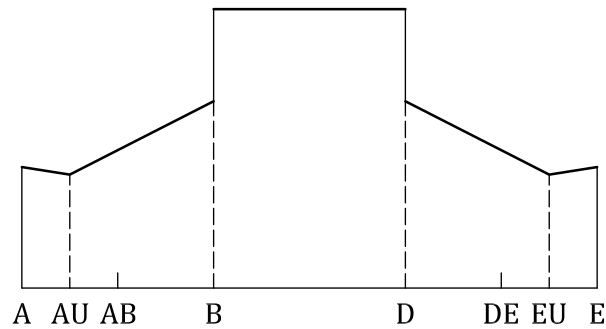
Figure 27 — Load sharing factor for cylindrical helical gears with \varepsilon_\beta \leq 0,8 and unmodified profiles, including buttressing effect
