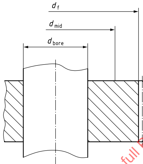
Figure 9 — Definitions of various diameters
