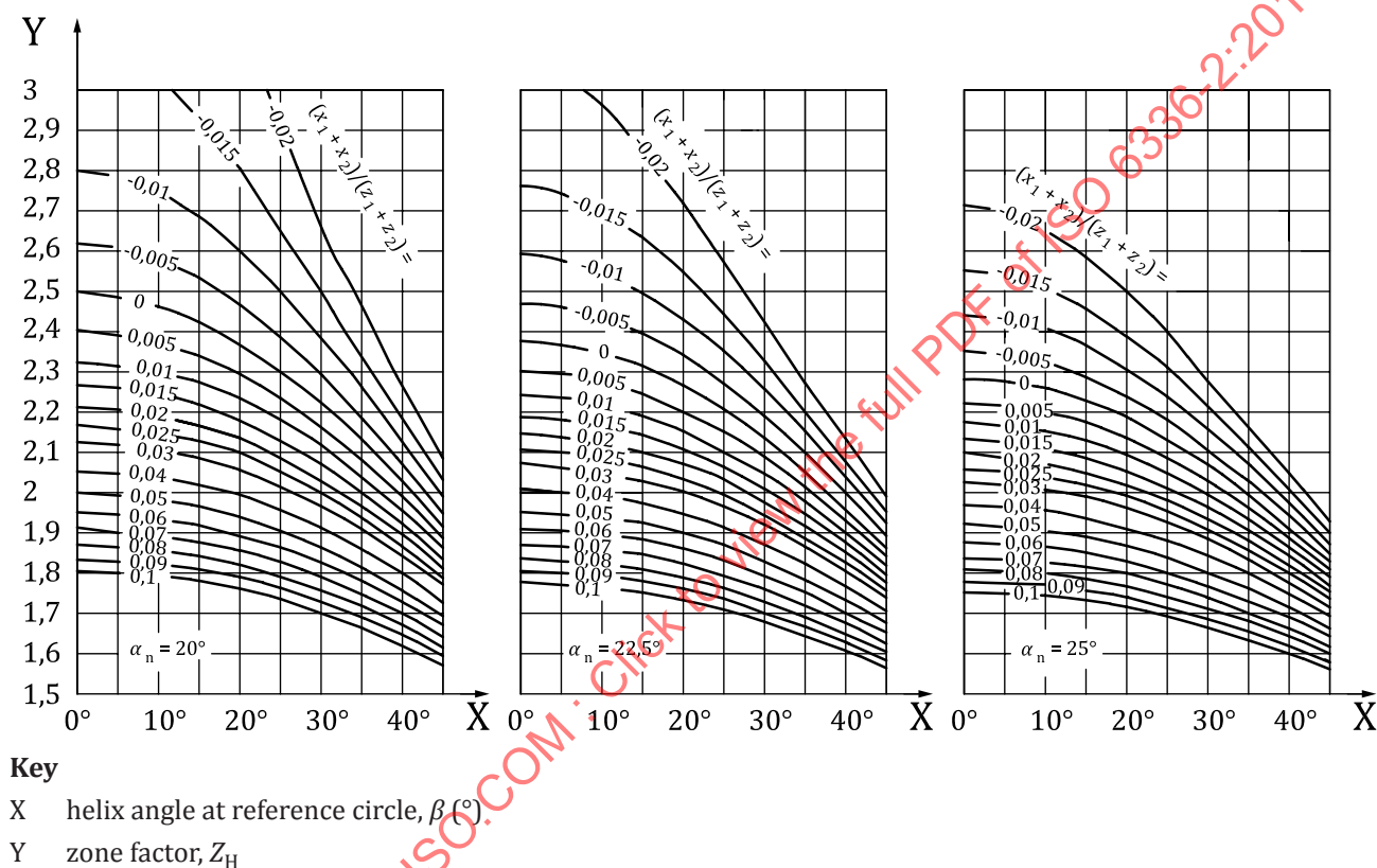
Figure 2 — Zone factor, Z_H
