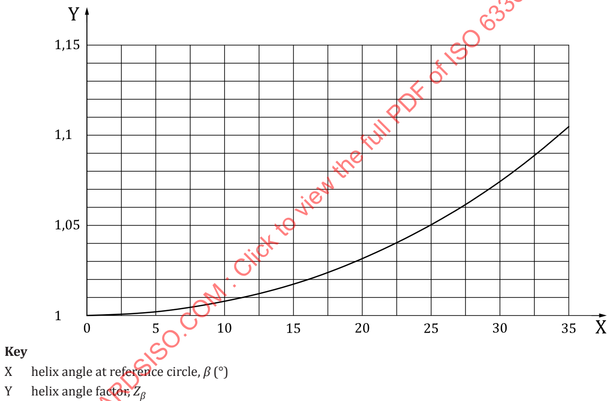
Figure 5 — Helix angle factor, Z_\beta
