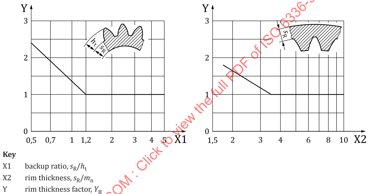
Figure 9 — Rim thickness factor, Y_B
