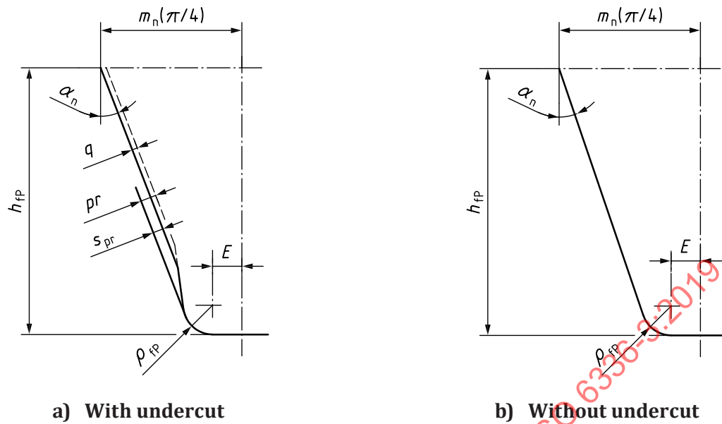
Figure 2 — Dimensions and basic rack profile of the teeth (finished profile)
