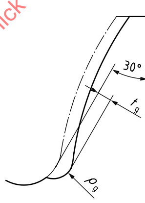
Figure 7 — Notch dimensions if the notch is near the critical section
