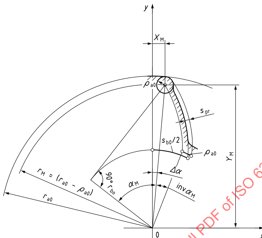
Figure 6 — Quantities at the shaper cutter
