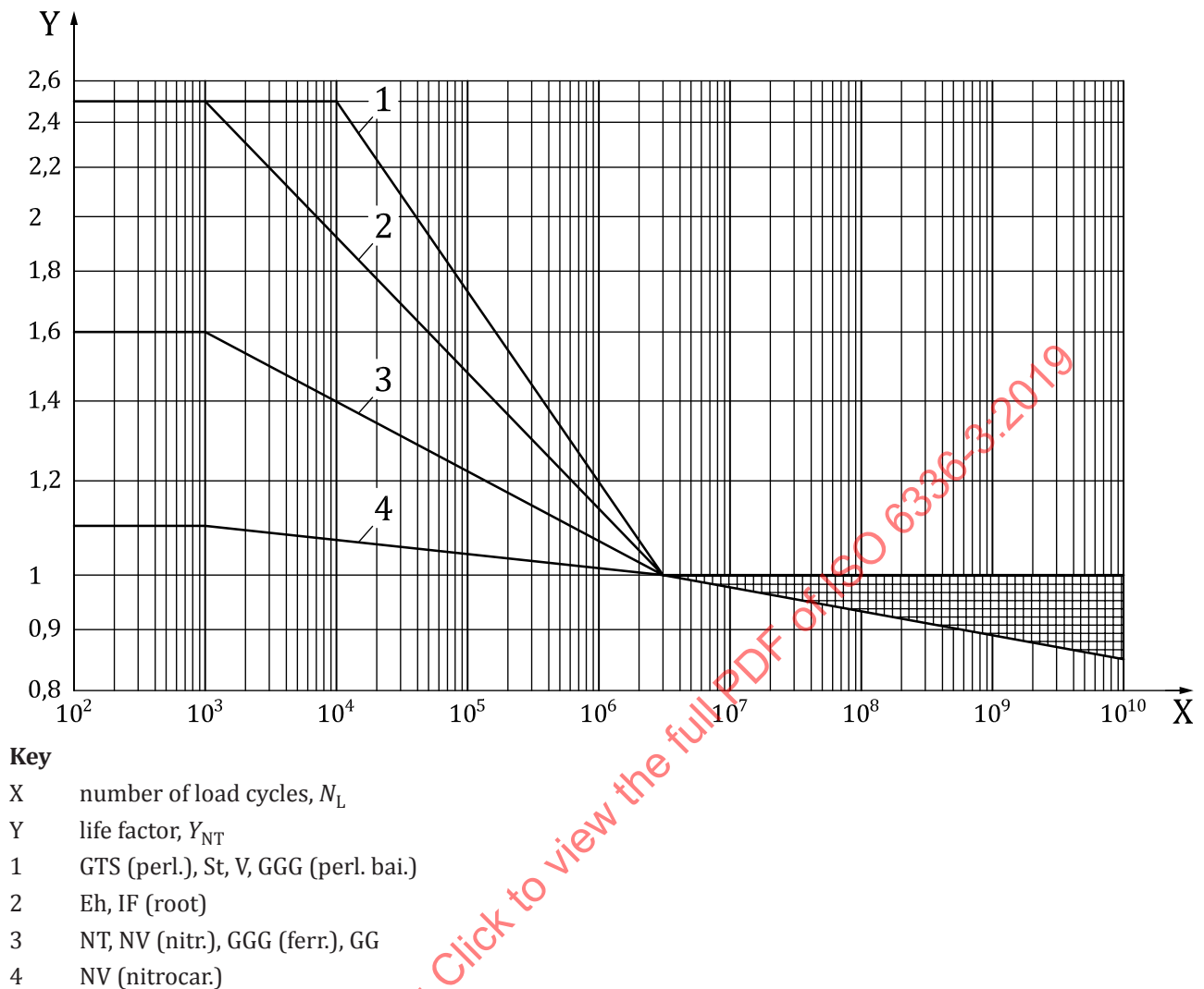
Figure 11 — Life factor, Y_{NT} , for reference test gears
