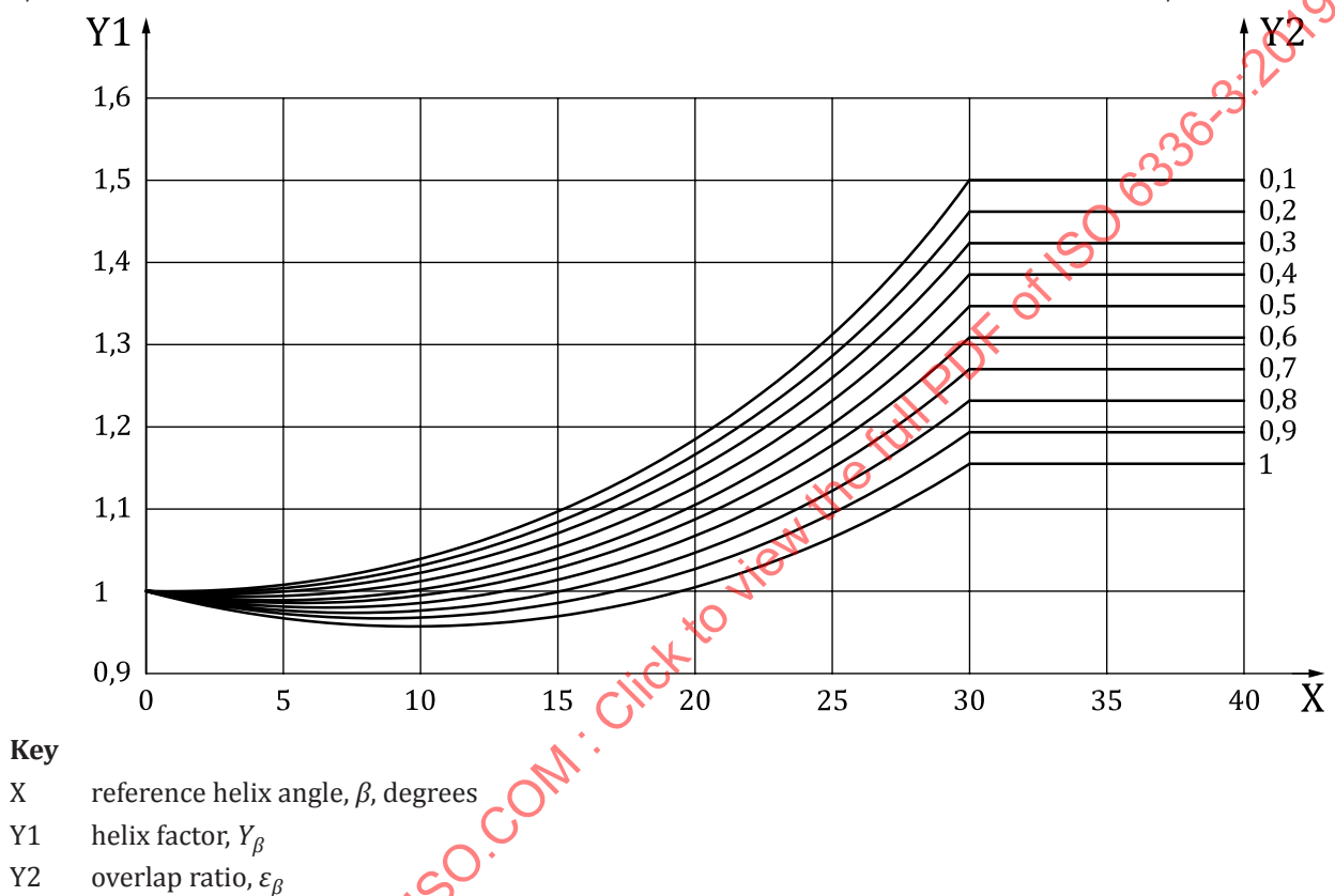
Figure 8 — Helix factor, Y_\beta
