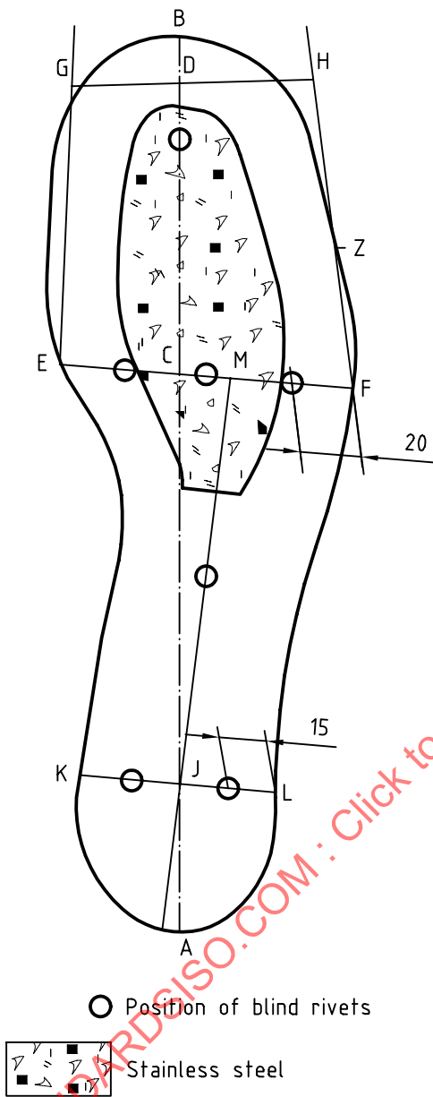
Figure A.1 — Insole pattern
