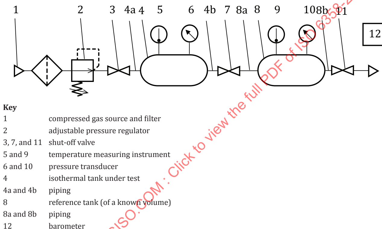
Figure B.1 — Test circuit
