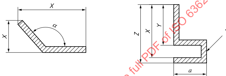
Figure 3 — Sectional dimensions
