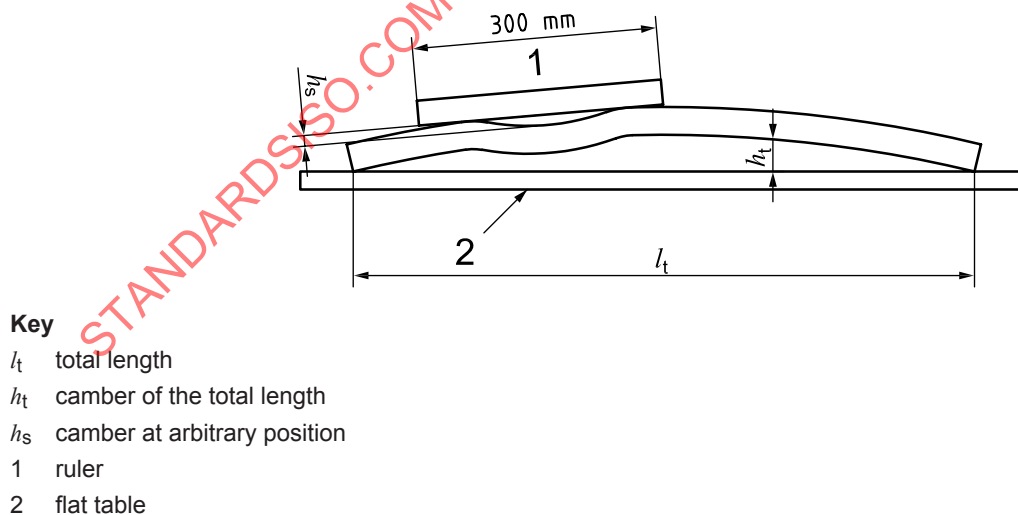
Figure 5 — Straightness
