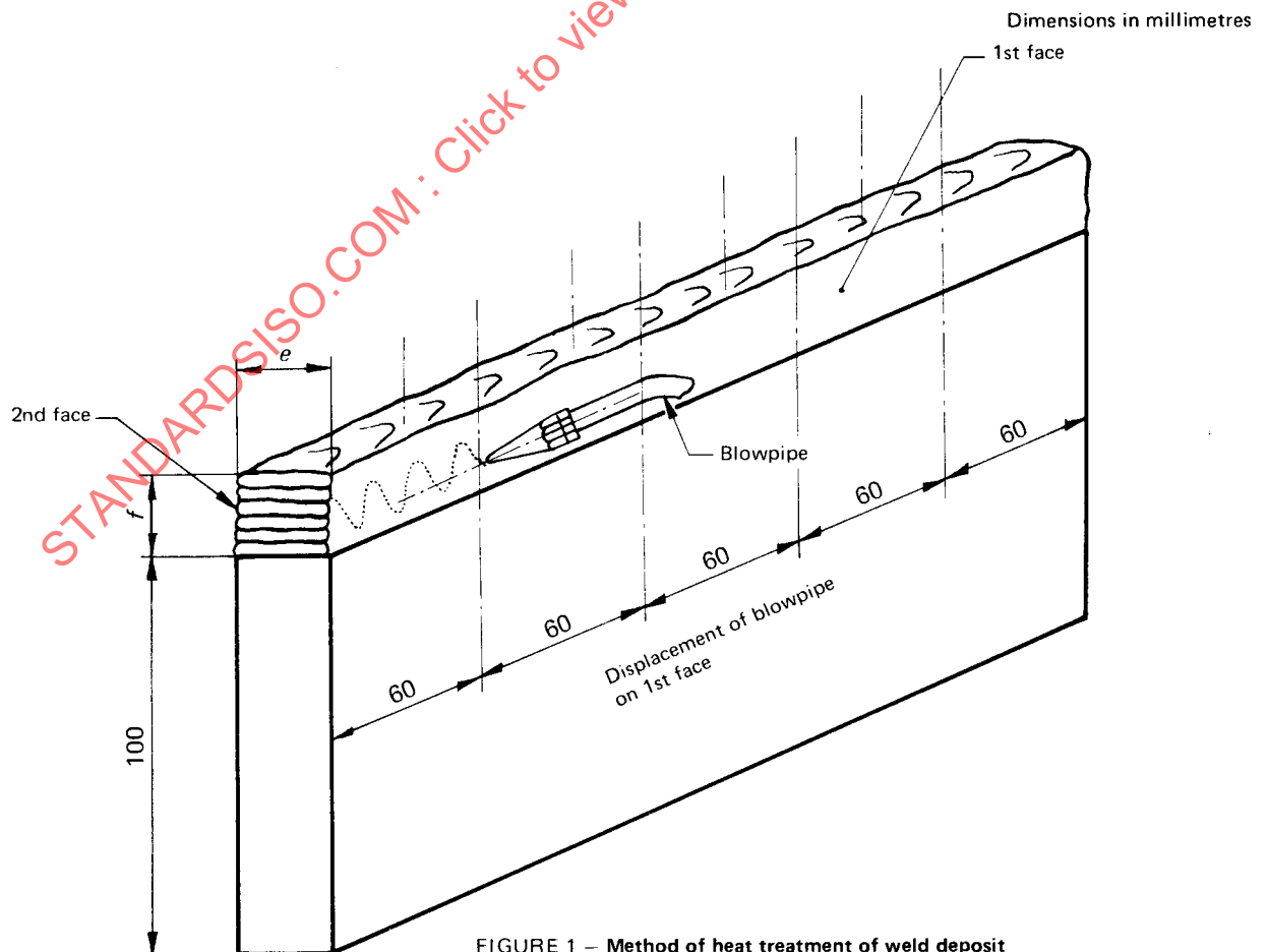
FIGURE 1 — Method of heat treatment of weld deposit
