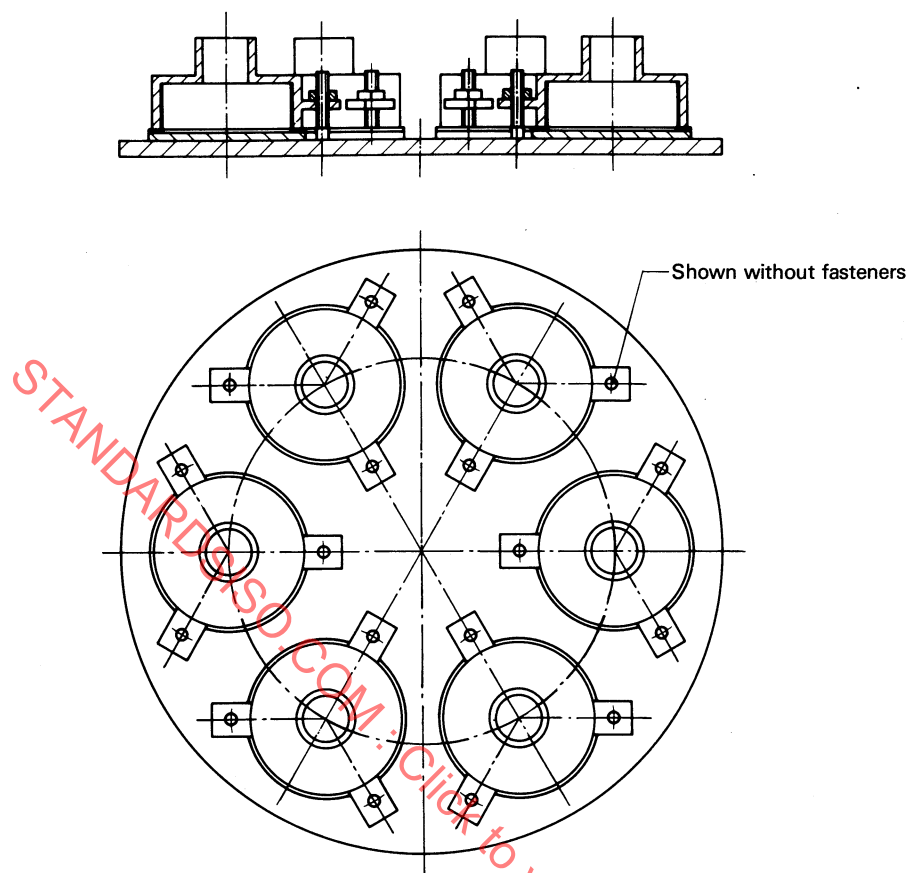
Figure 1 — Arrangement of the specimens and reference glass plates in the abrasion testing apparatus
