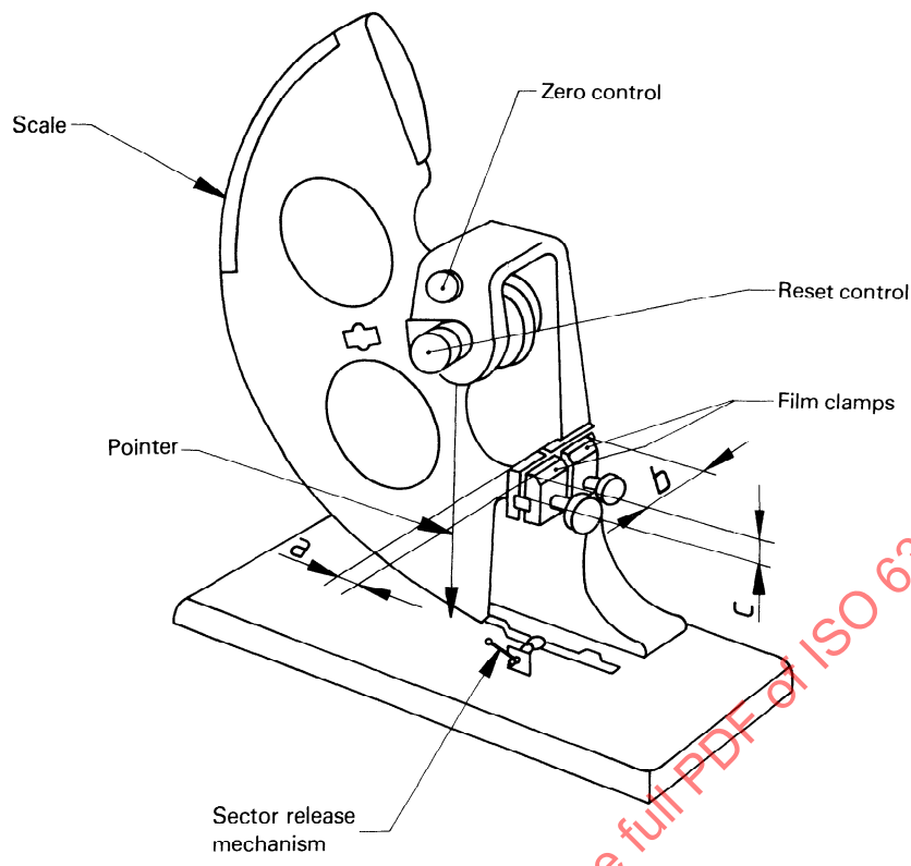
Figure 1 — Elmendorf tear test apparatus
