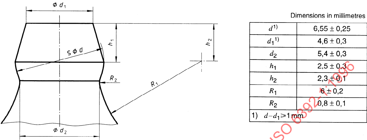
Figure 2 — Detailed dimensions of fitting head
