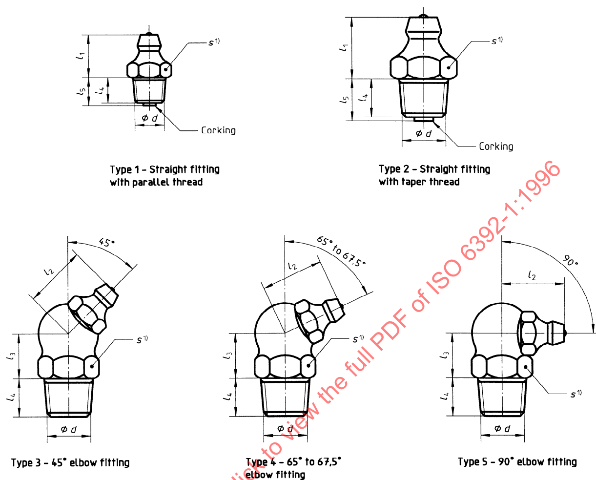
Figure 1 — Types of fitting
