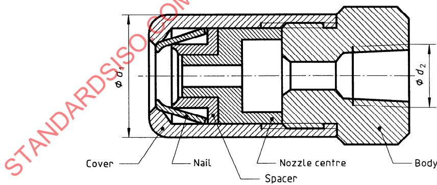
Figure 2 — Rubber nozzle-centre type
