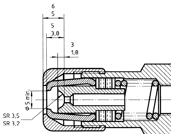
Figure A.2 — Steel nozzle-centre type
