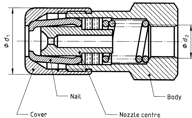
Figure 3 — Steel nozzle-centre type
