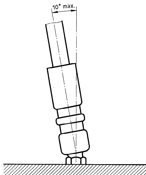
Figure 4 — Injection angle
