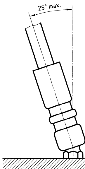
Figure 5 — Uncoupling angle
