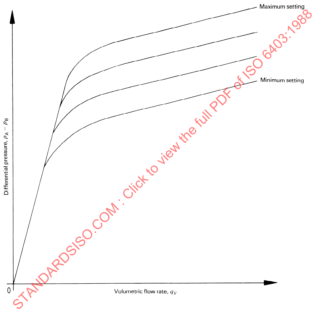
Figure 16 — Graphical representation of steady-state pressure/flow characteristics for pressure-relief valves
