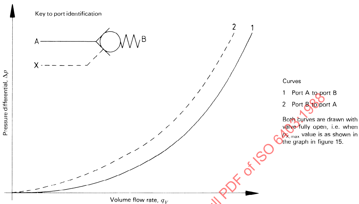
Figure 14 — Graphical representation of pressure/flow characteristics of pilot-pressure-operated non-return valves
