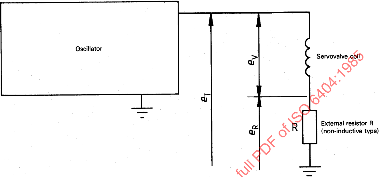
Figure 4 — Servovalve coil impedance test
