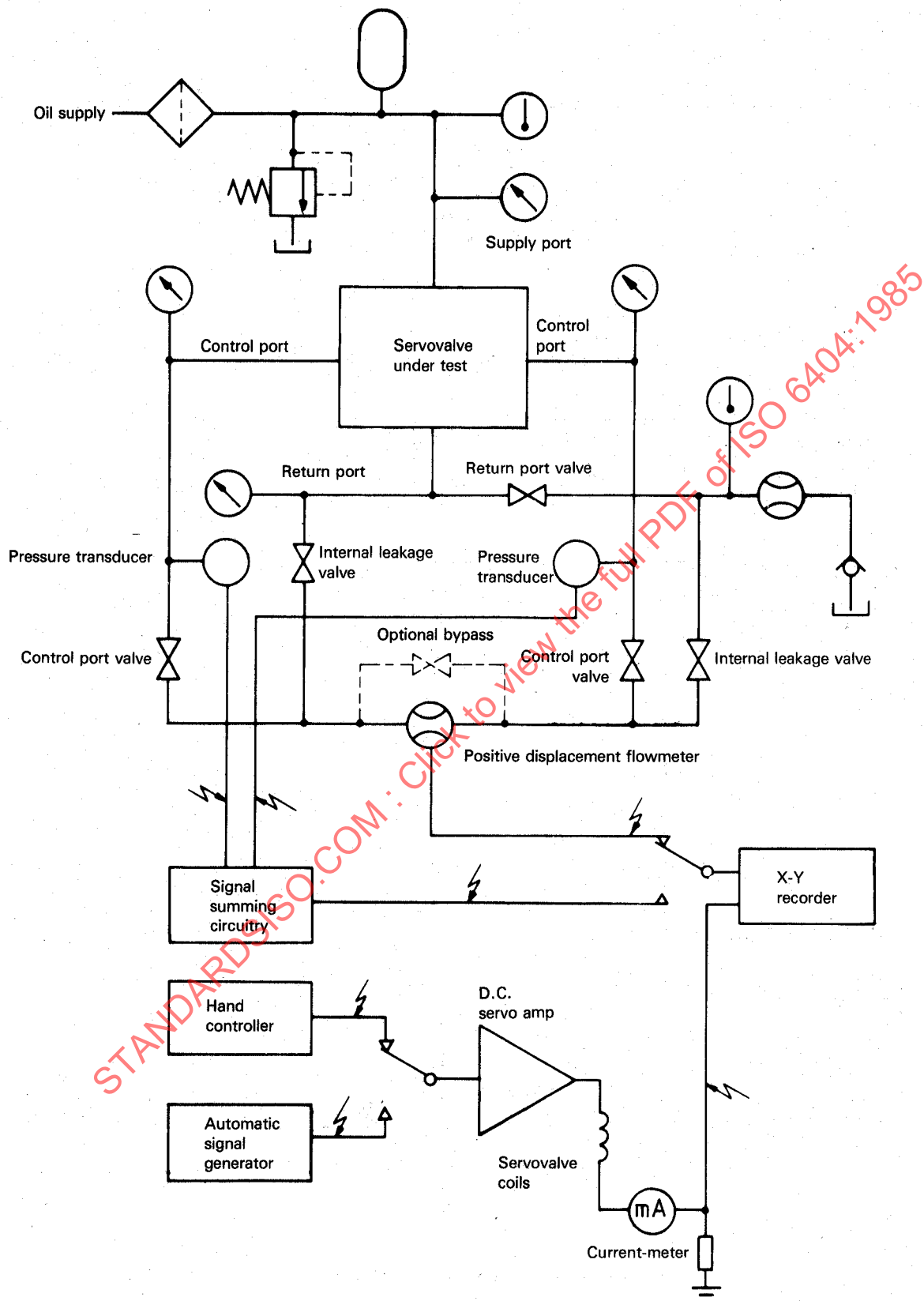
Figure 1 — Steady-state test circuit 1)
