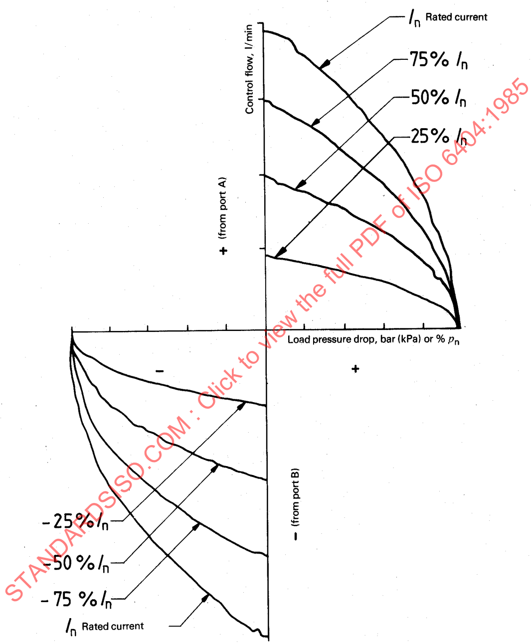
Figure 9 — Control flow versus load pressure drop
