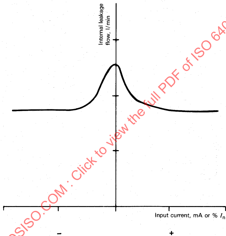
Figure 8 — Internal leakage versus input current
