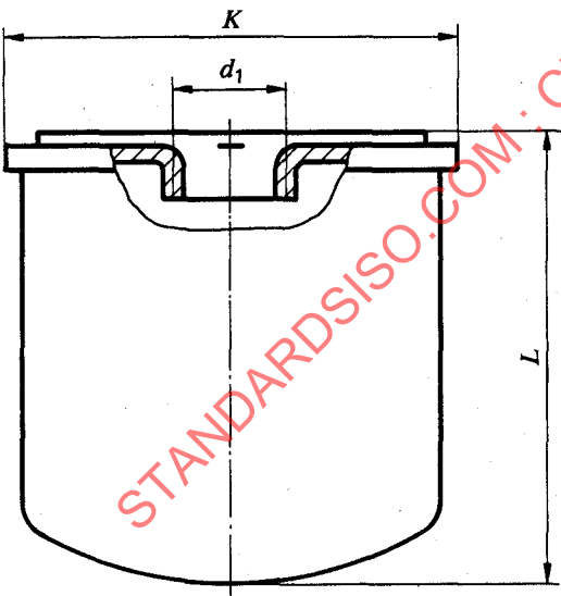
Figure 2 — Filter
