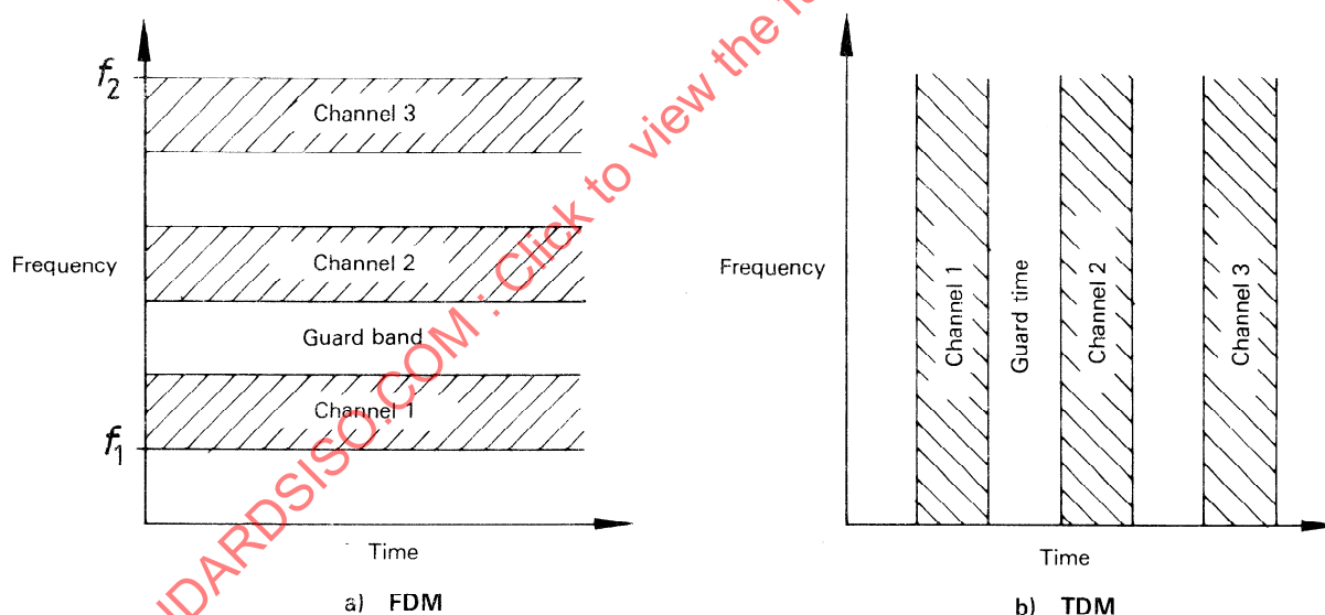
Figure 8 — Frequency and time division multiplexing
