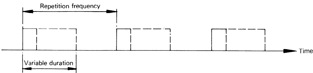
Figure 4 — Pulse duration modulation (PDM)
