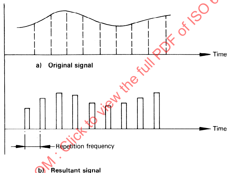
Figure 5 — Pulse amplitude modulation (PAM)
