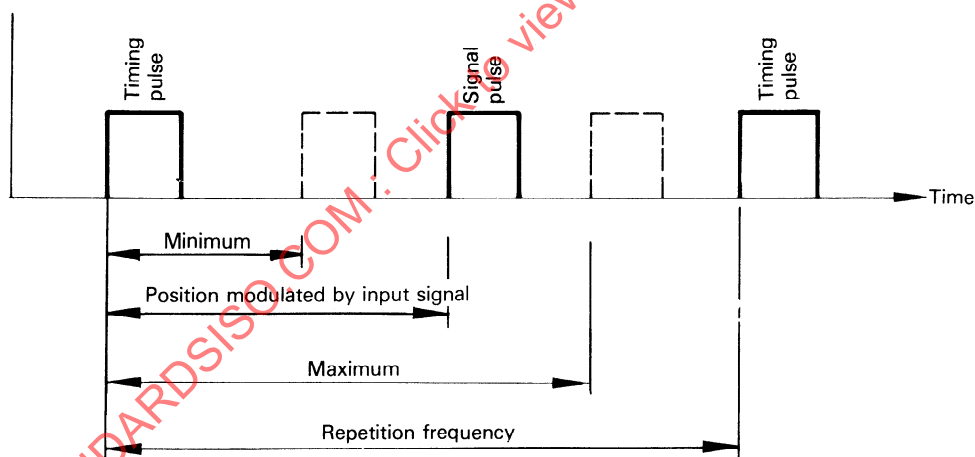
Figure 7 — Pulse position modulation (PPM)
