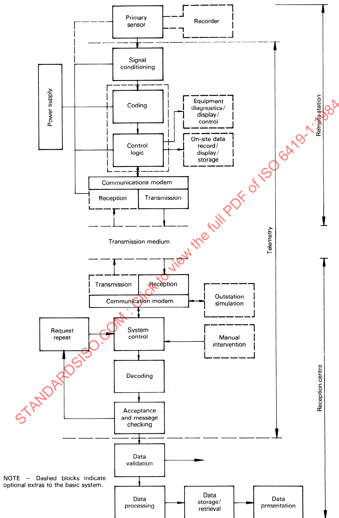
Figure 1 — Data acquisition system — Functional block diagram
