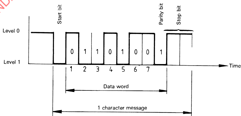
Figure 6 — Pulse code modulation (PCM) (Illustrates an 8-bit character)
