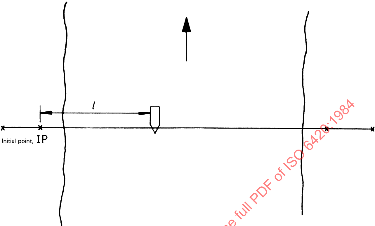
Figure 1 — Position fixing for stream gauging
