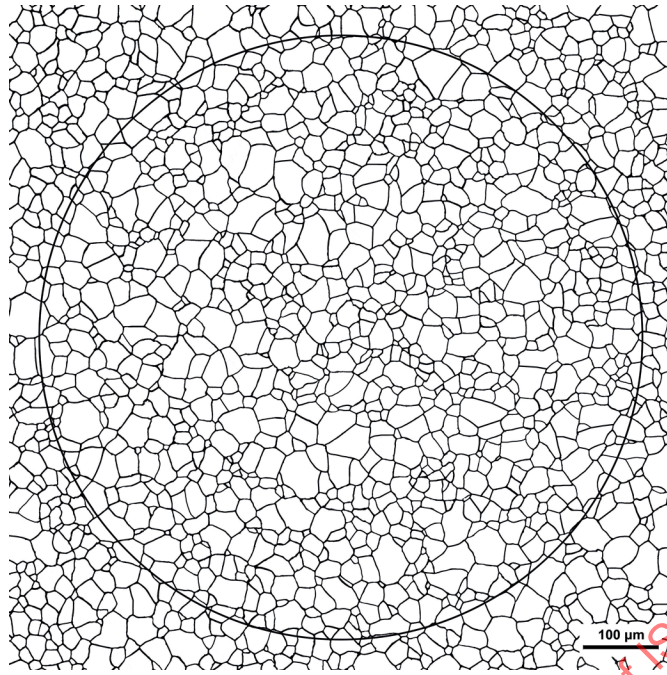
Figure B.18 — Grain size 8
