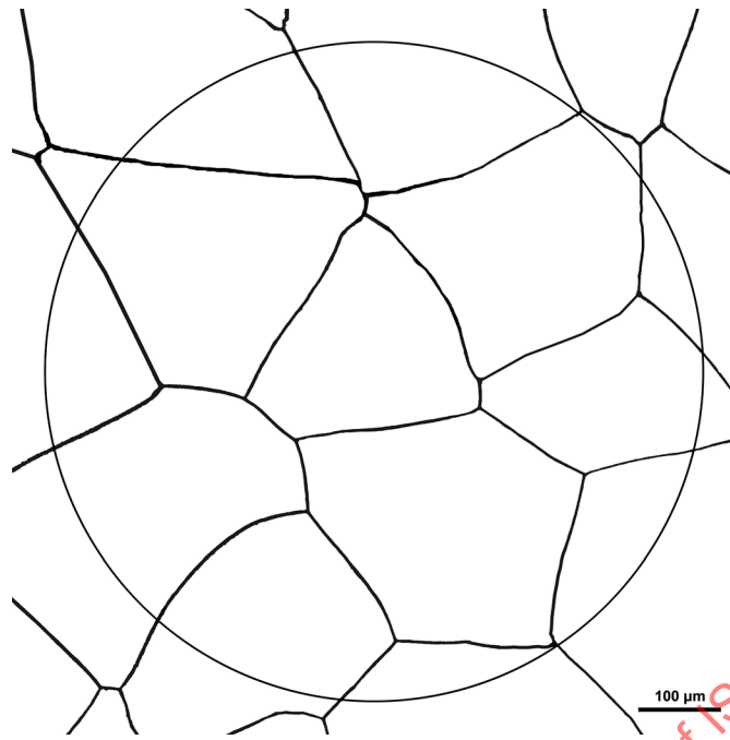
Figure B.4 — Grain size 1
