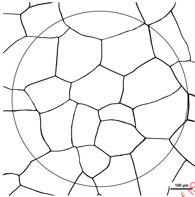
Figure B.6 — Grain size 2
