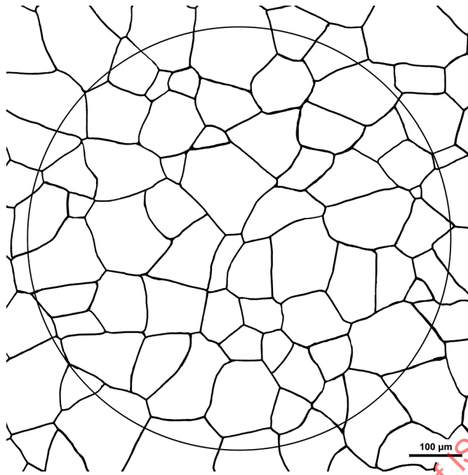
Figure B.10 — Grain size 4
