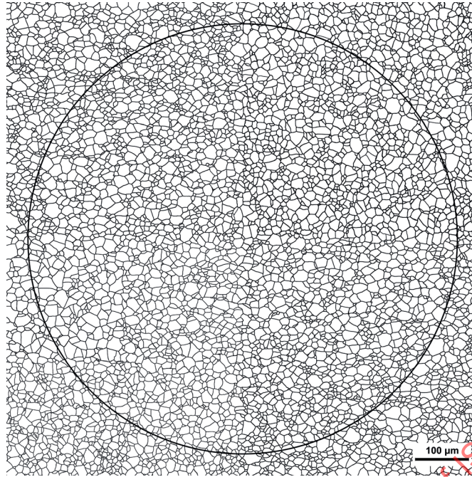
Figure B.22 — Grain size 10
