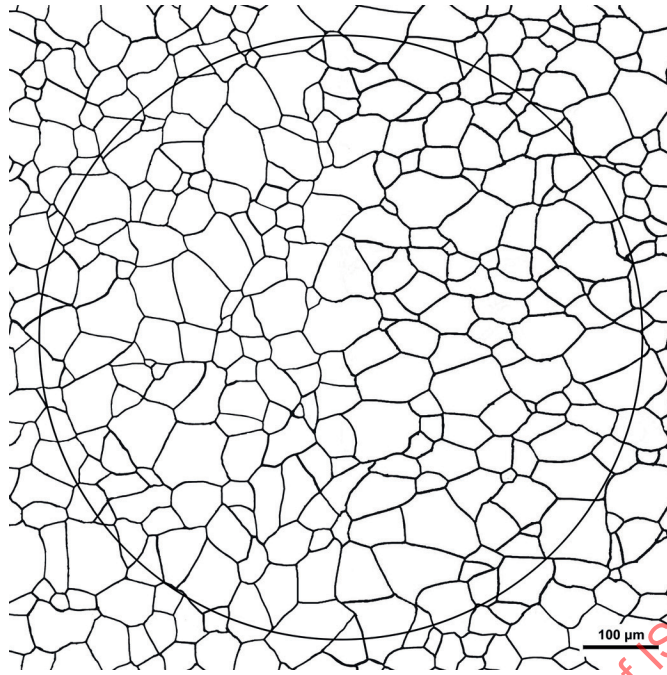
Figure B.14 — Grain size 6
