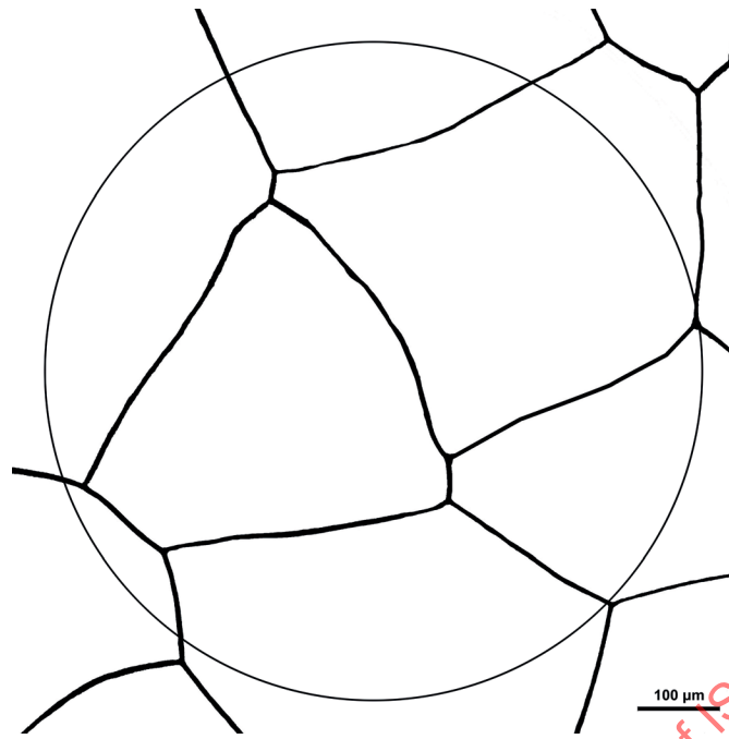
Figure B.2 — Grain size 0
