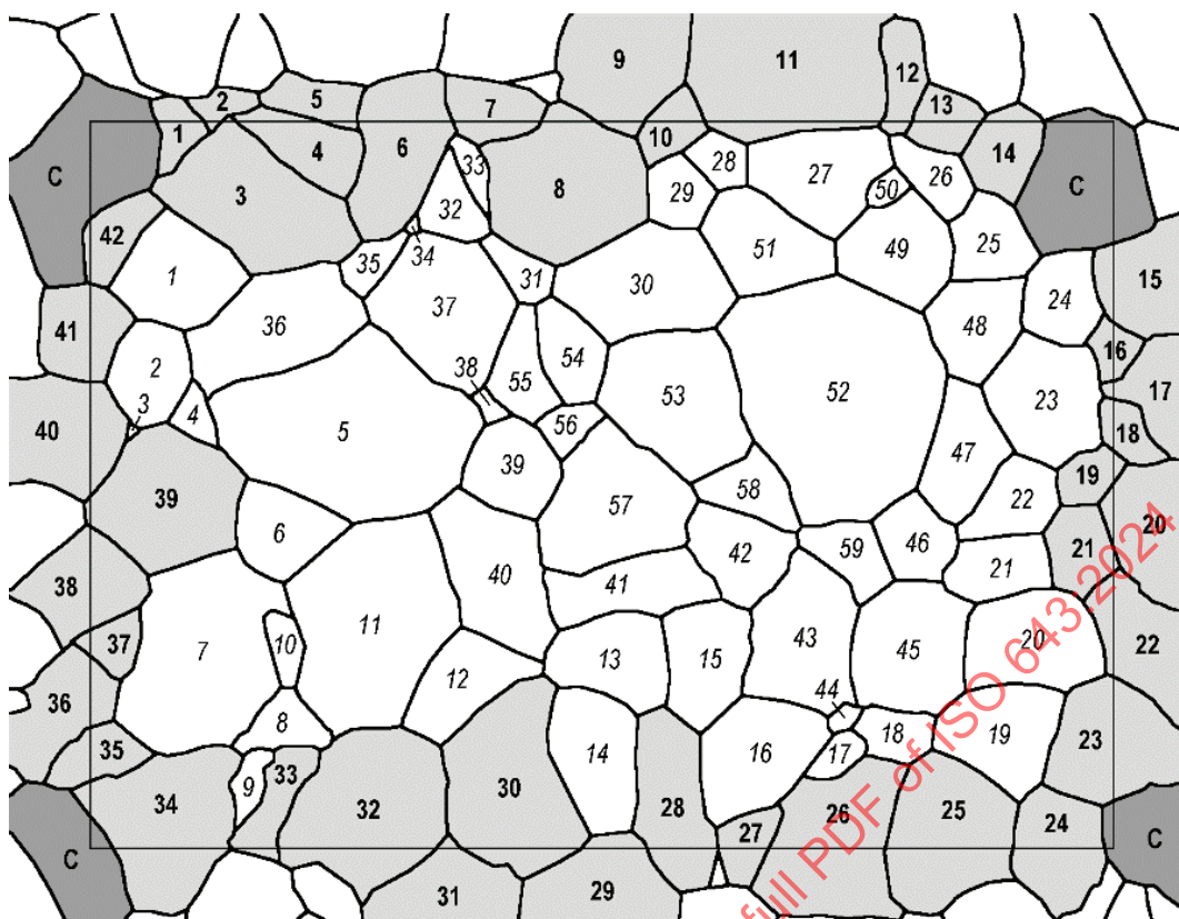
Figure 4 — Evaluation of the number of grains in an area enclosed by a square or rectangle
