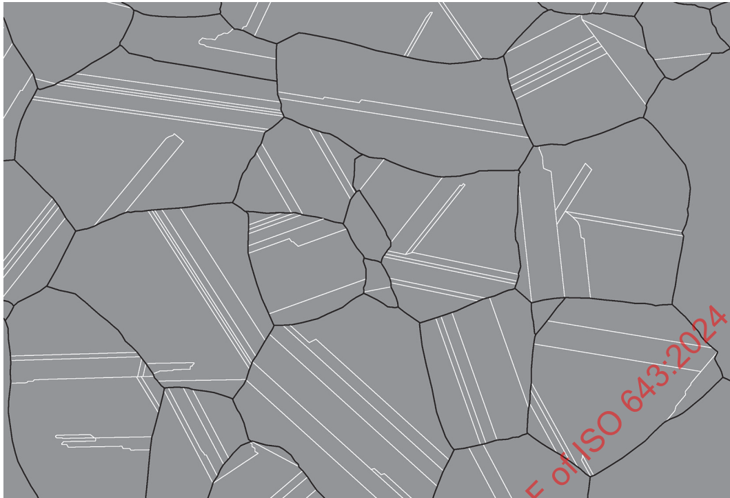
Figure 6 — Evaluation of number of grains (twin grains)
