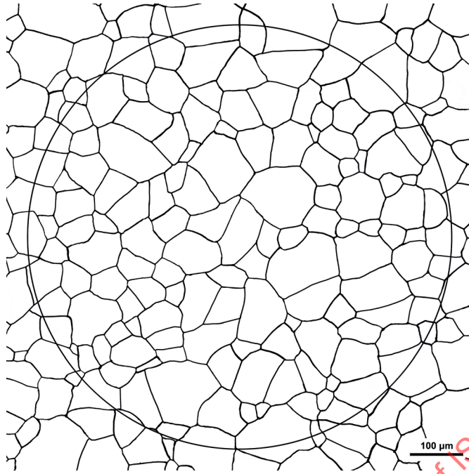
Figure B.12 — Grain size 5
