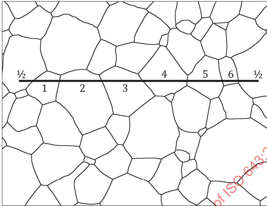
Figure 1 — Example of intercept, N
