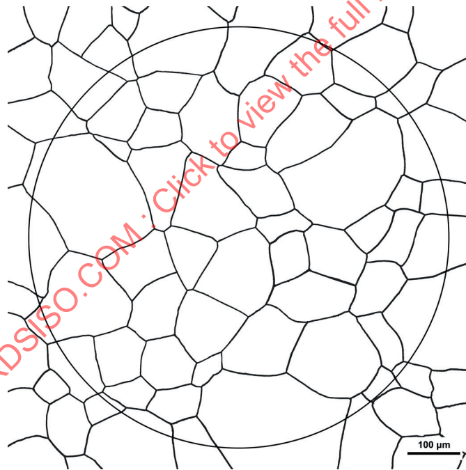
Figure B.9 — Grain size 3,5
