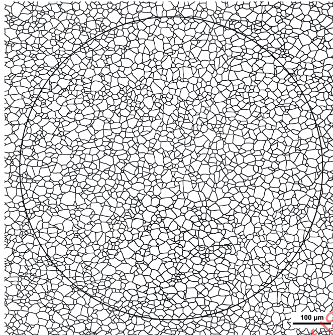
Figure B.20 — Grain size 9
