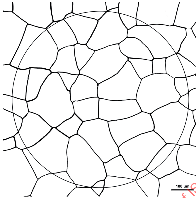
Figure B.8 — Grain size 3
