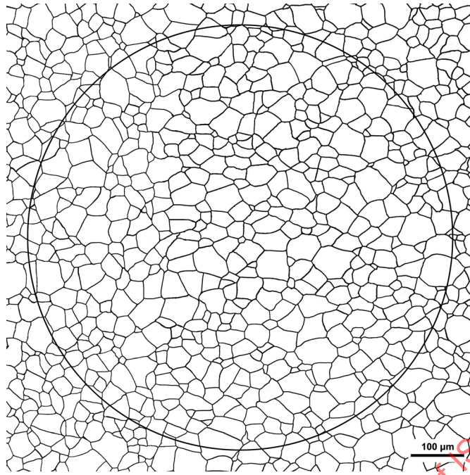
Figure B.16 — Grain size 7
